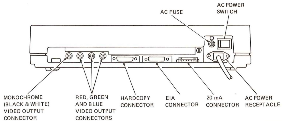
FIGURE 3-1 Terminal Controls
