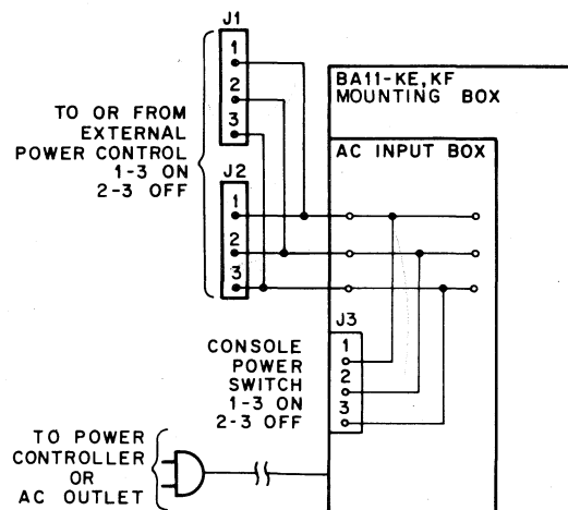
Figure 3-3 Power Control
