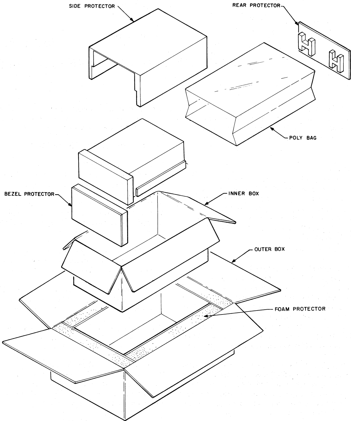
Figure 3-1 BA11-K Packaging
