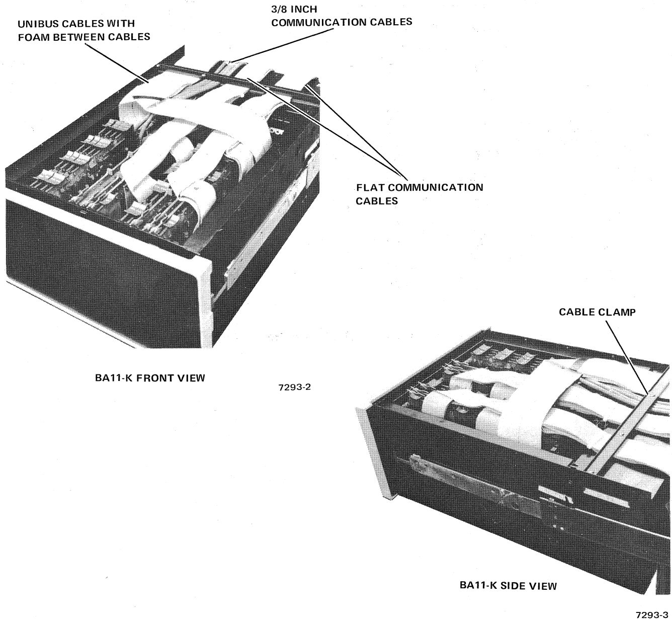
Figure 2-5 Cable Routing
