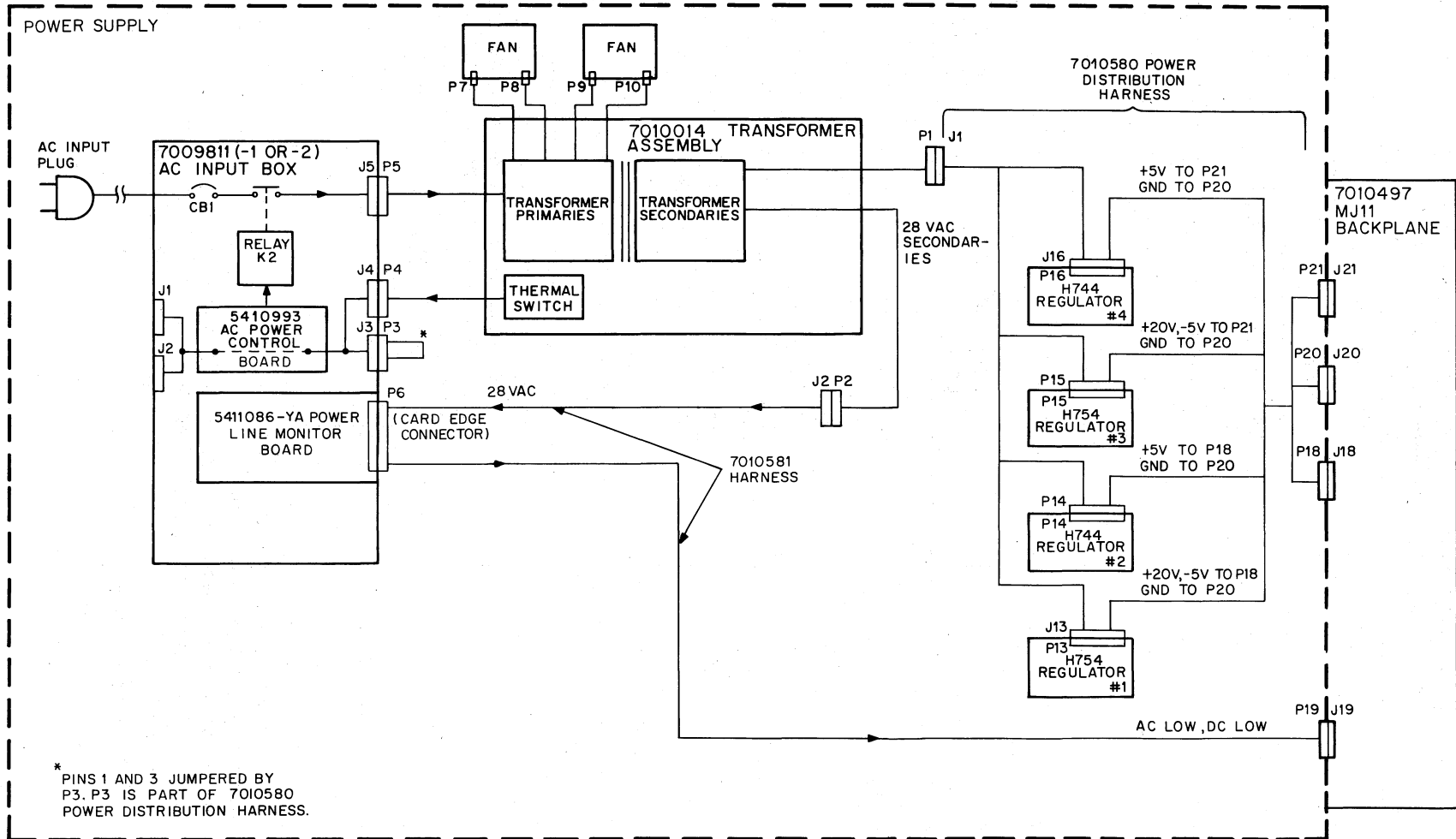
Figure 4-30 MJ11 Power Supply Functional Block Diagram
