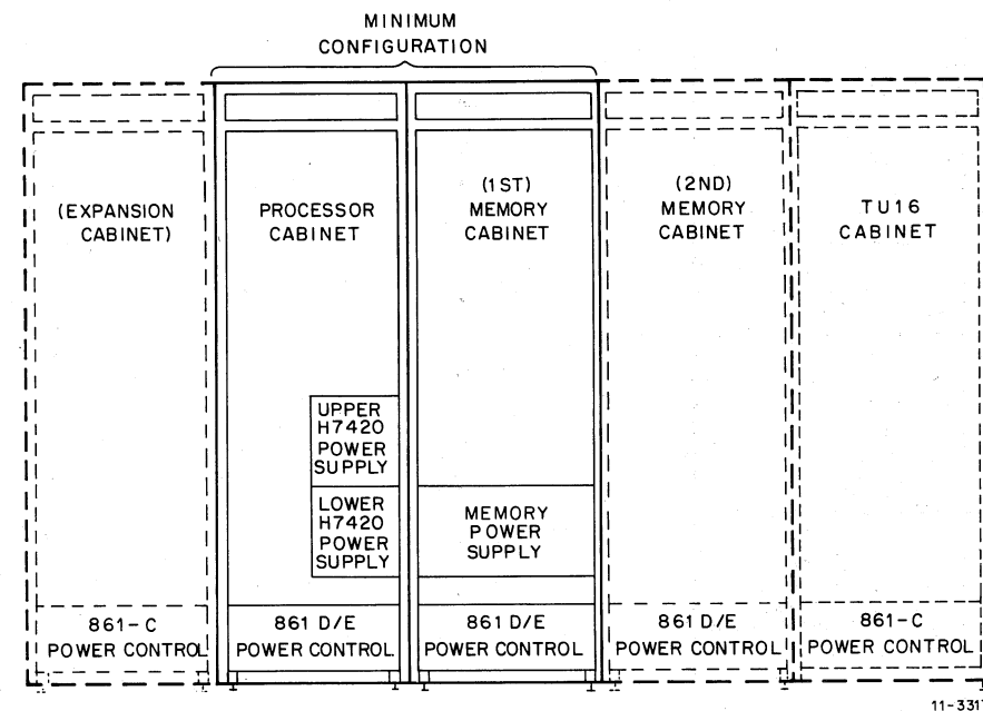
Figure 4-1 PDP-11/70 Power System, Physical Location
