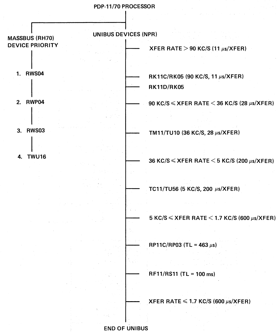
Figure 3-32 PDP-11/70 Configuration
