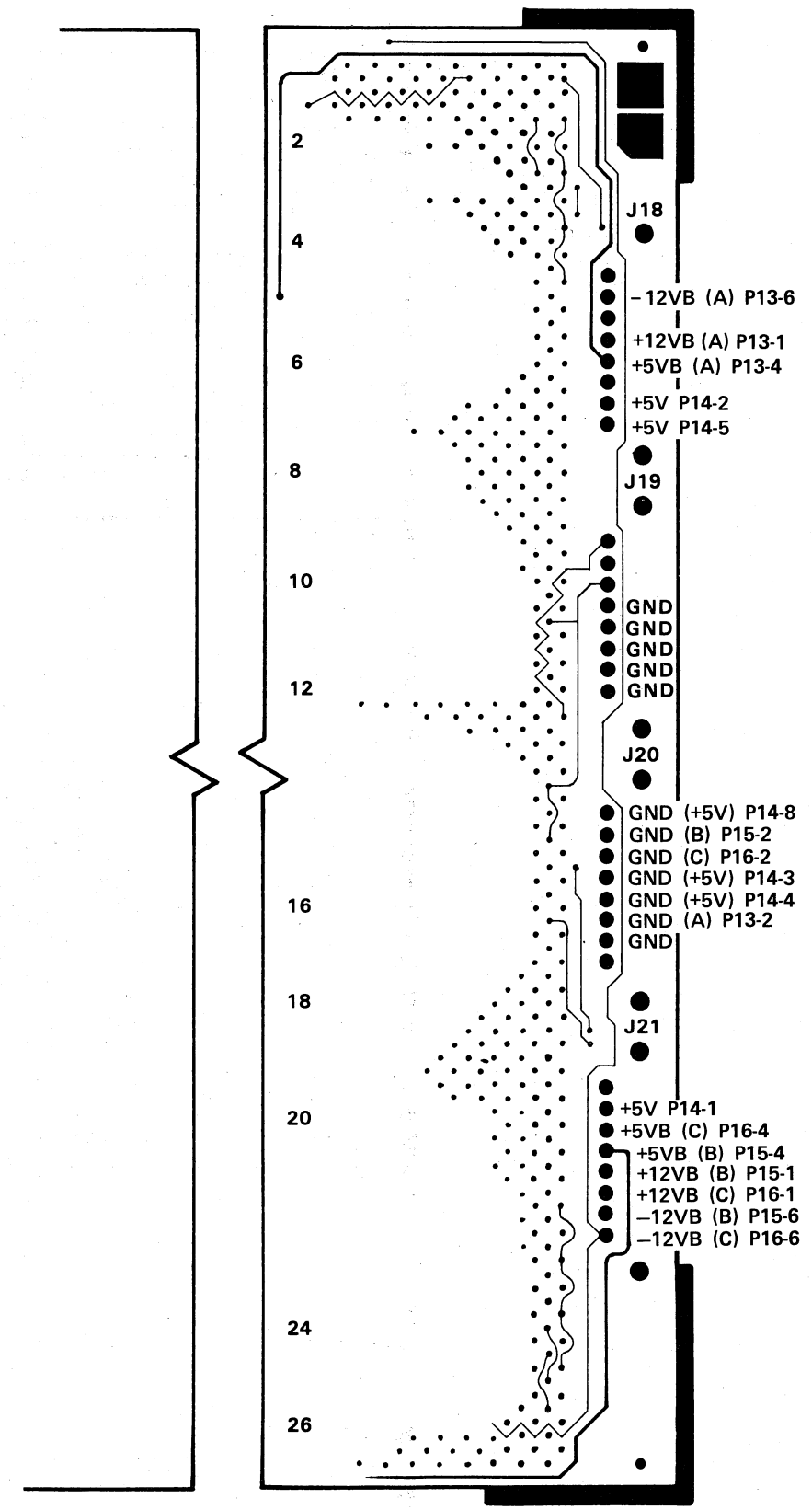
Figure 4-45 MK11 Backplane Power Connections
