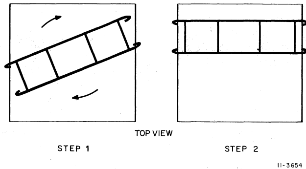
Figure G-7 Positioning Horizontal Trough Section
