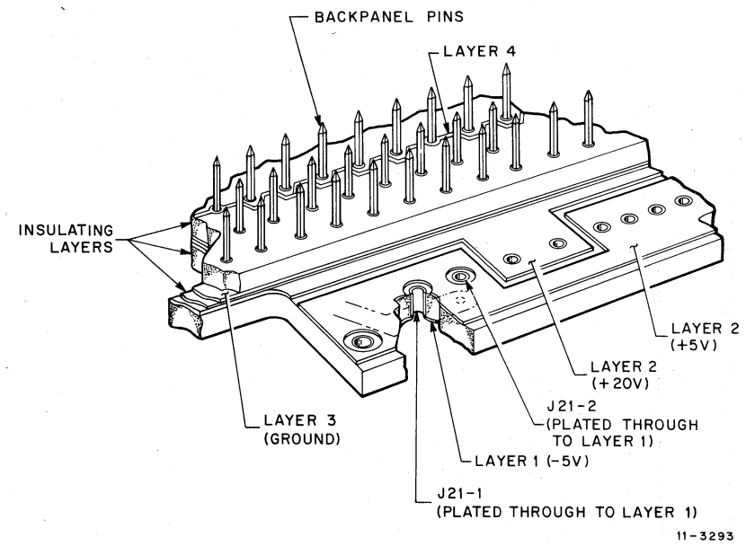
Figure 4-23 Memory Backplane Cross Section
