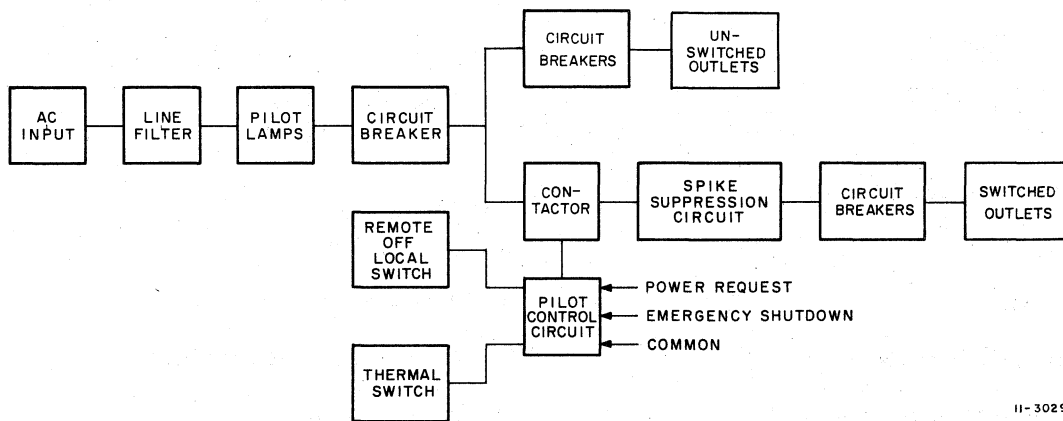
Figure 4-6 861 Power Controller Simplified Block Diagram
