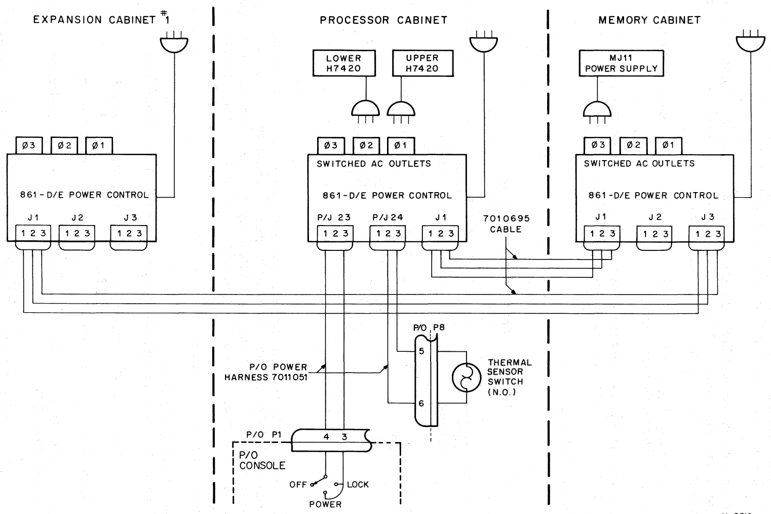
Figure 4-10 Example of Remote Power Control
