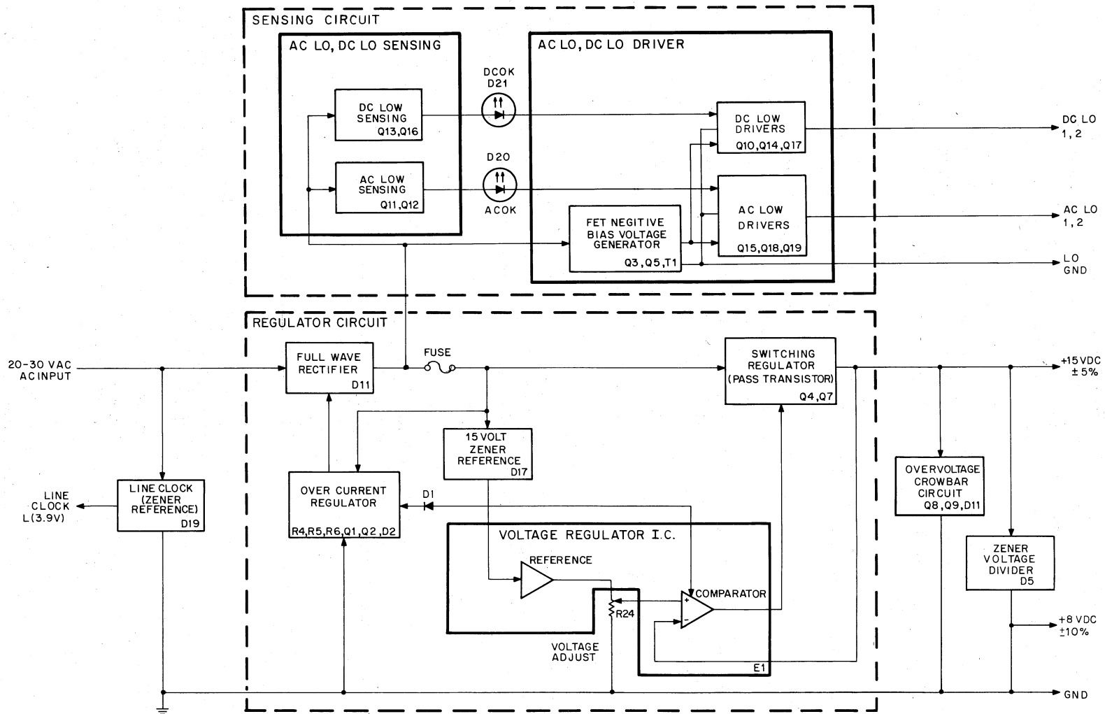
Figure 4-34 5411086 Block Diagram
