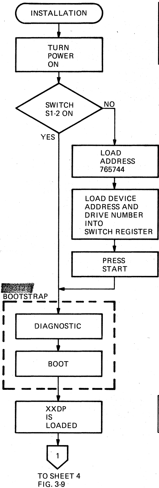
Figure 3-9 System Checkout (Sheet 3 of 4)
