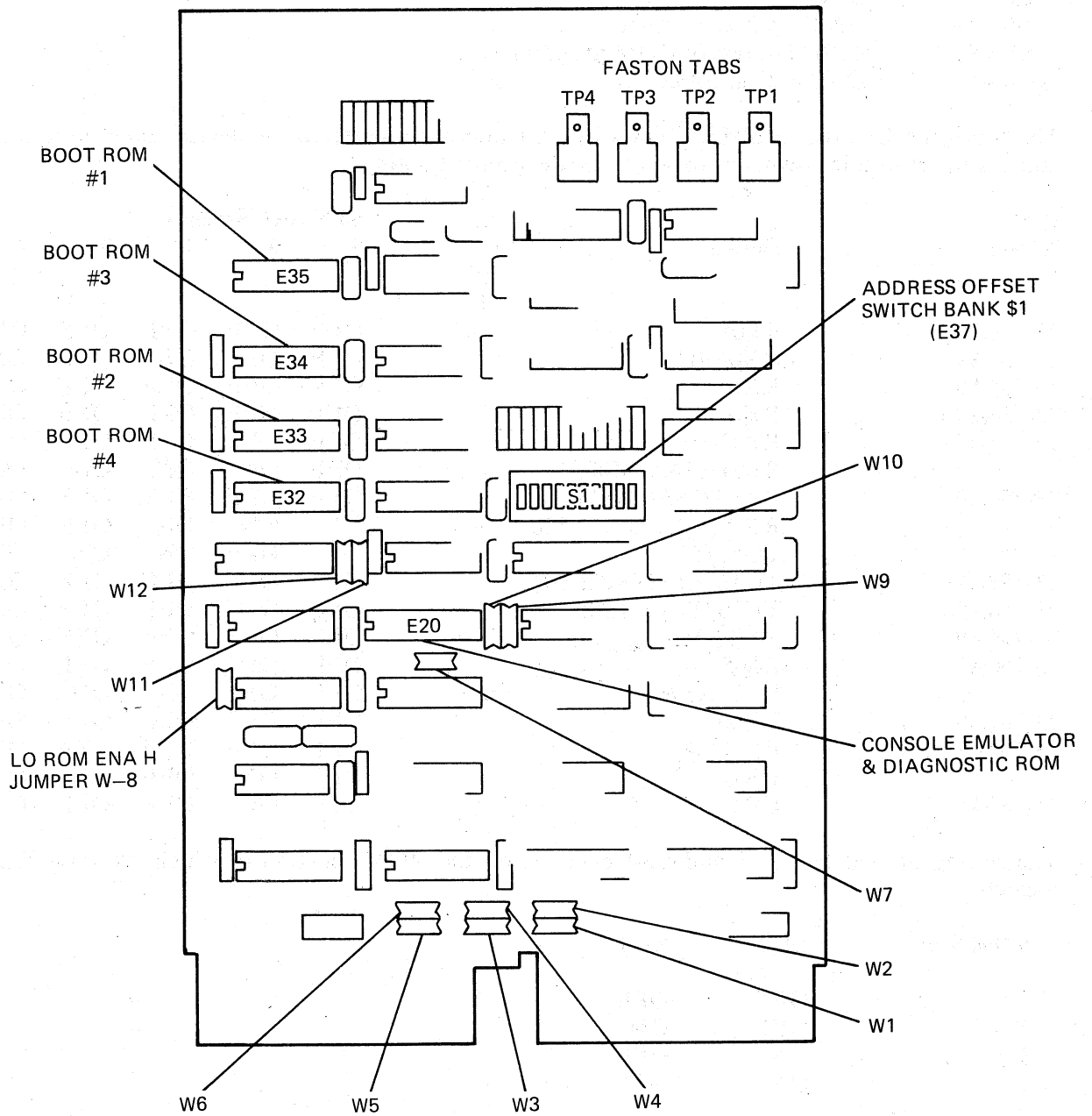
Figure 3-13 M9312 Bootstrap/Terminator Module
