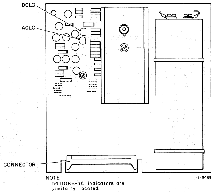
Figure 5-12 5411086 AC LO and DC LO Indicators
