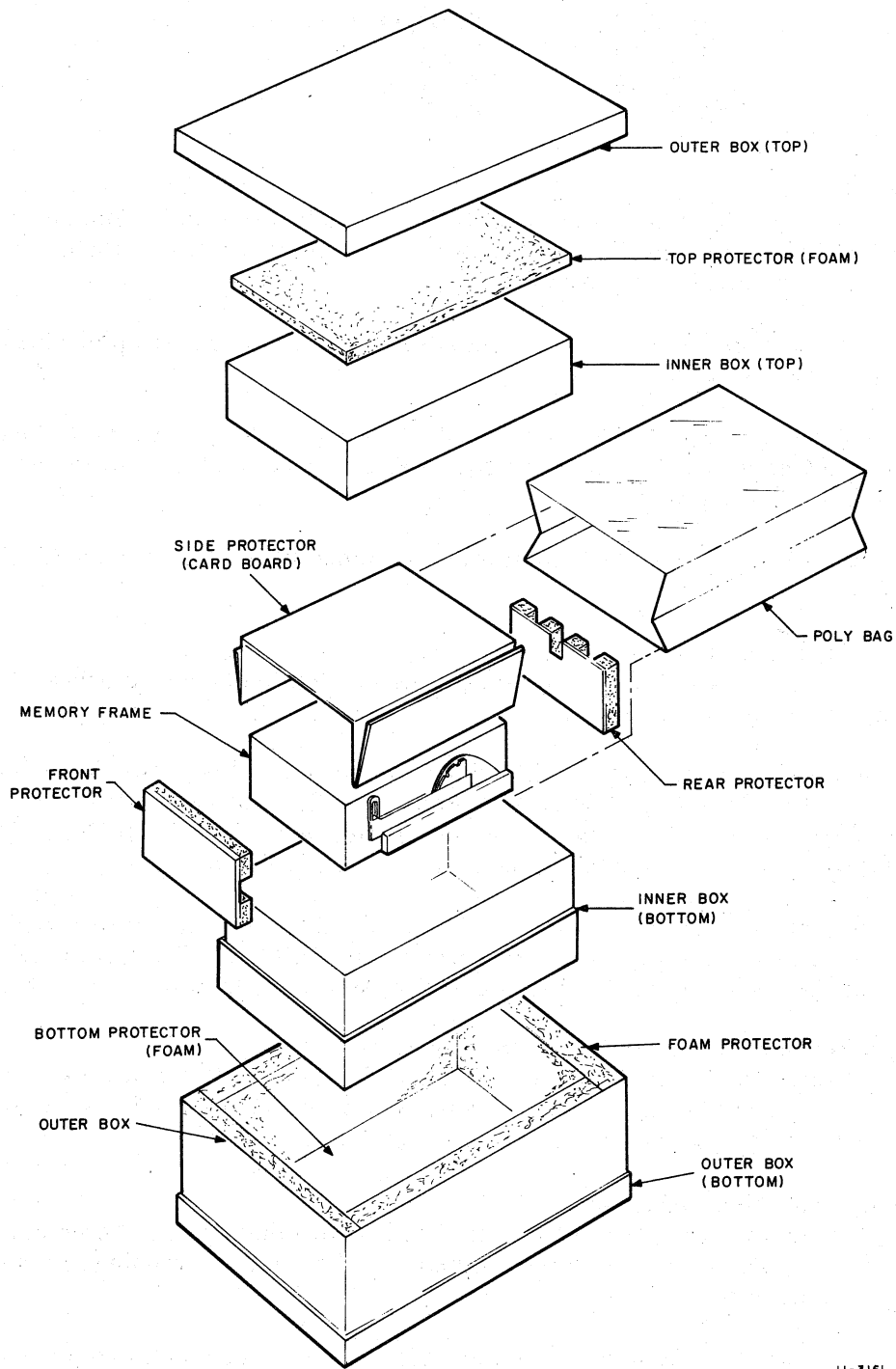
Figure 3-14 Memory Frame Packaging
