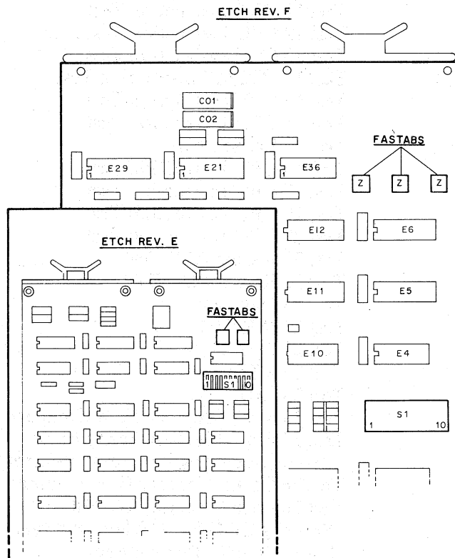
Figure 3-11 M9301-YC Etch Revisions
