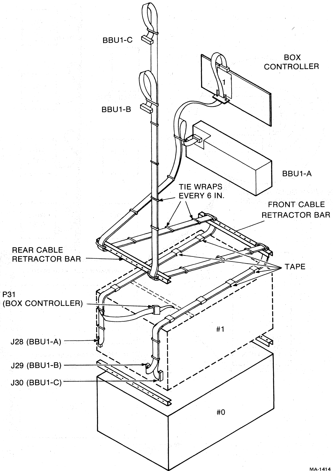
Figure 3-24 Box Controller and Battery Backup Power Cables
