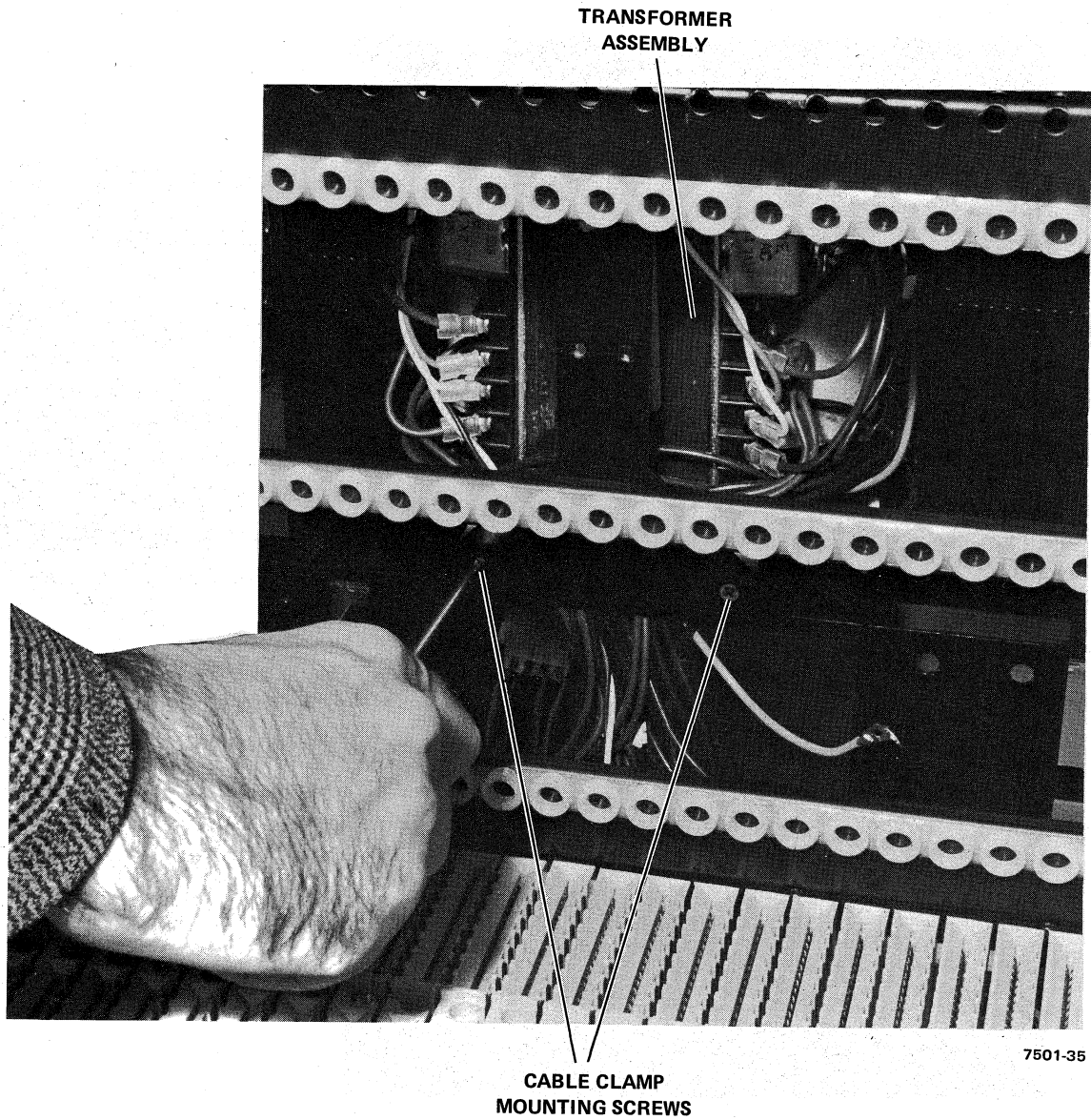
Figure 4-62 Transformer Assembly Removal (Sheet 1 of 2)
