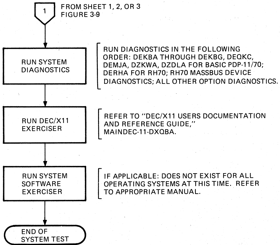
Figure 3-9 System Checkout (Sheet 4 of 4)
