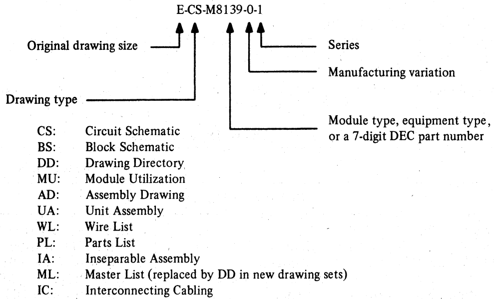
Figure 1-4 Drawing Nomenclature
