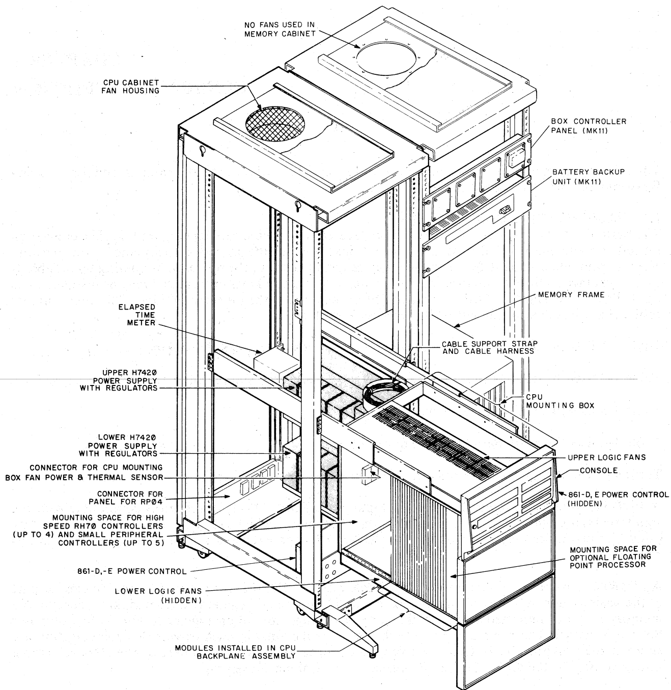
Figure 1-1 Location of Major Components and Assemblies
