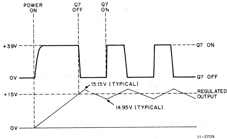
Figure 4-36 5411086 Regulator Waveforms
