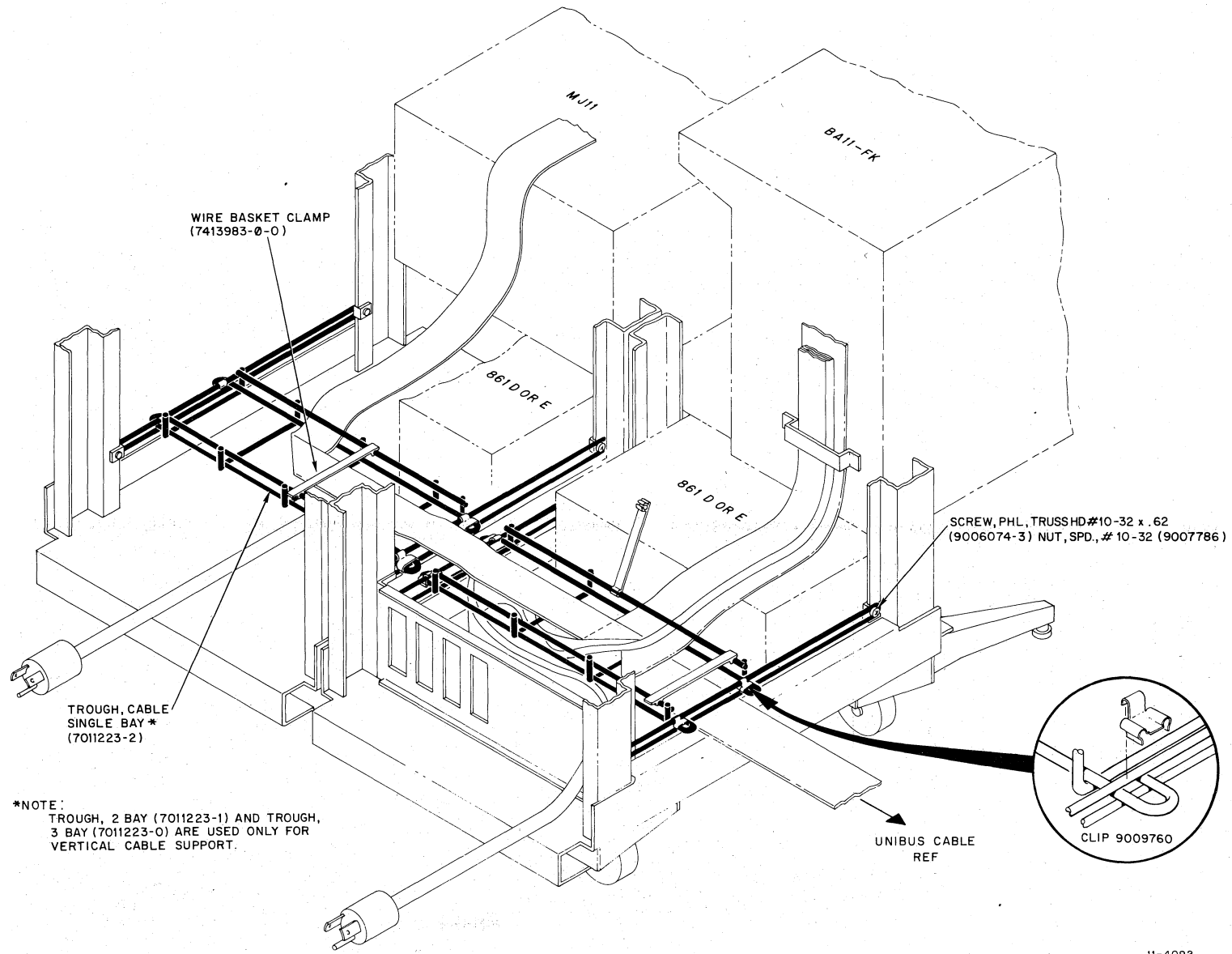
Figure G-2 PDP-11/70 with Cable Troughs
