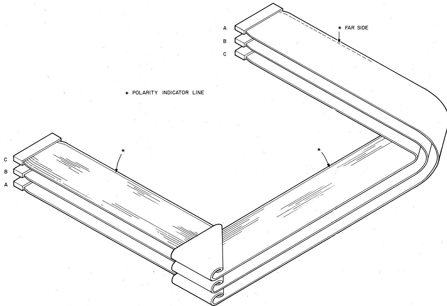
Figure G-10 TU16 Cables: Cables Inverted and Red Stripe on Same Side
