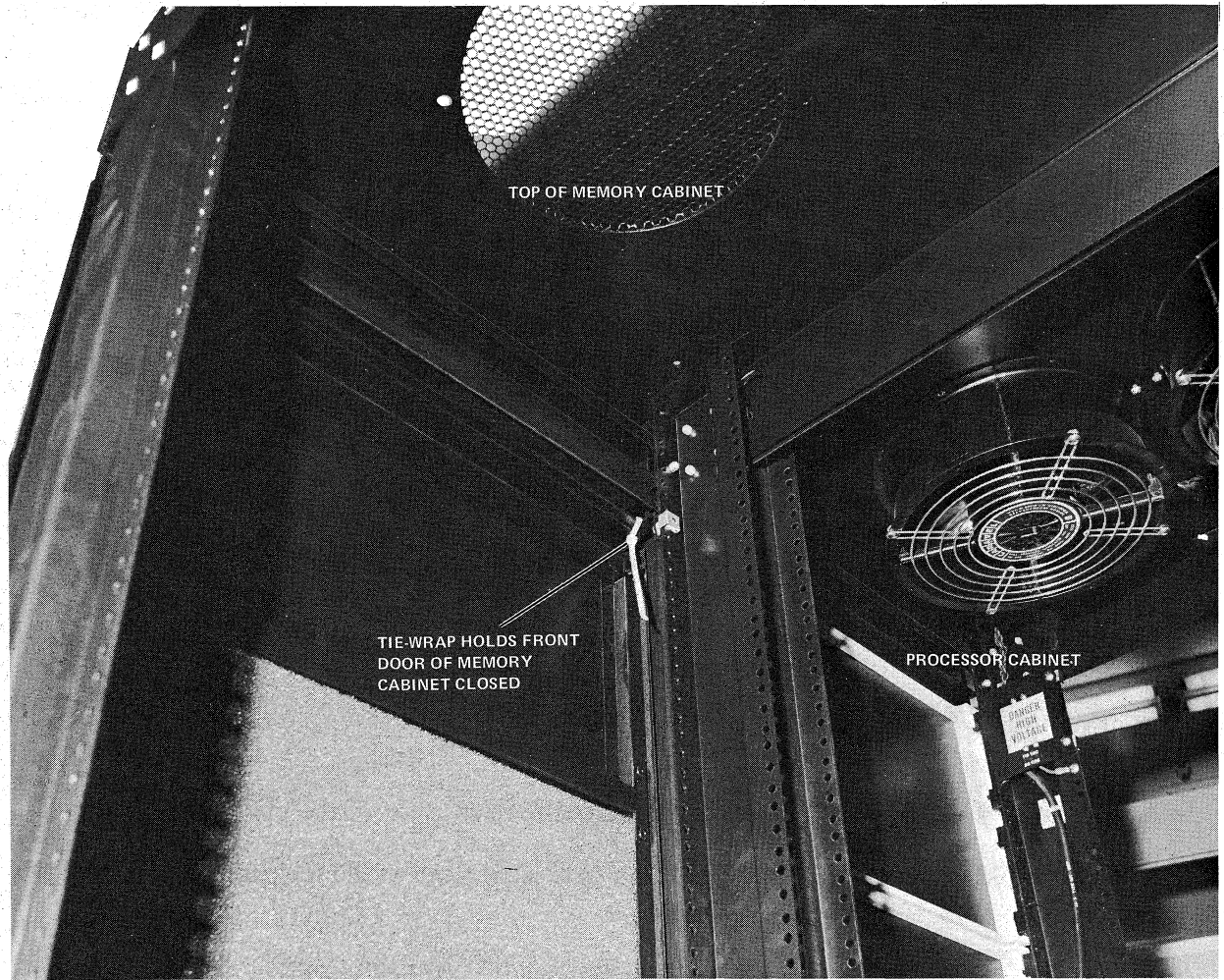
Figure 3-1 View of Inside Top of Memory Cabinet as Shipped
