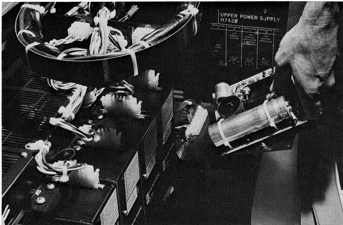
Figure 4-67 5411086 Removal (H7420) (Sheet 3 of 3)
