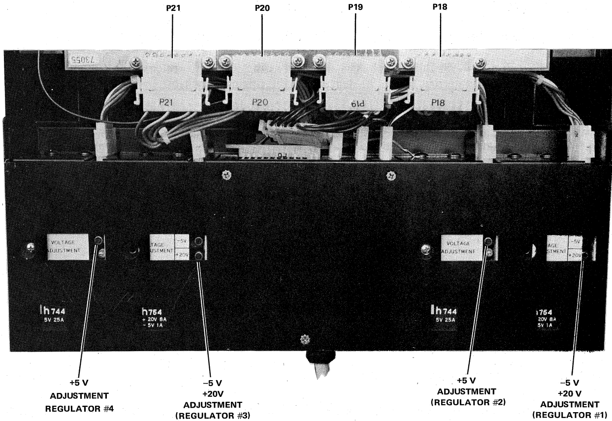
Figure 4-51 Regulator Adjustments
