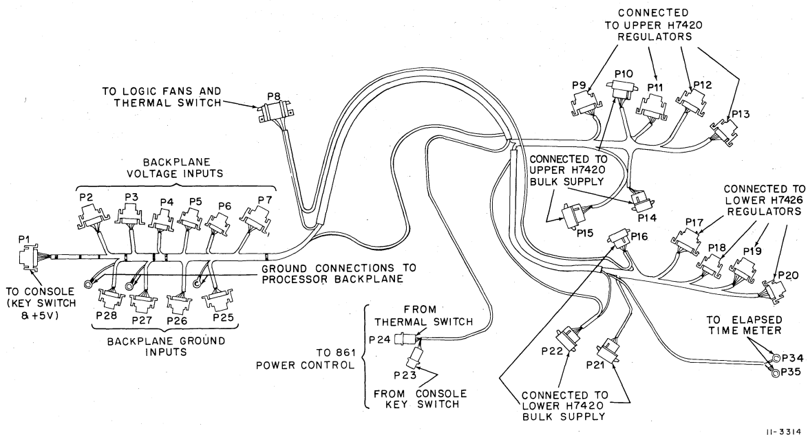
Figure 4-15 Power Distribution Cable Harness (Processor Cabinet) 7011051
