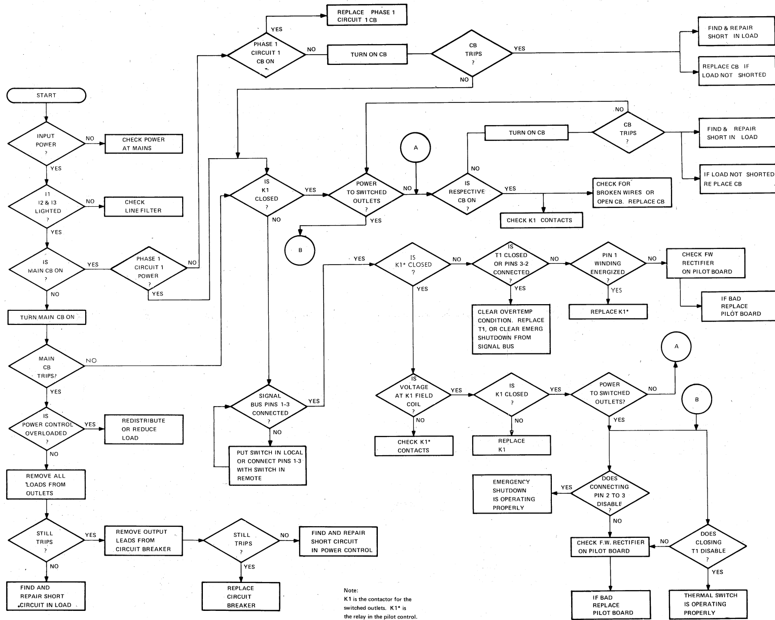
Figure 4-48 Troubleshooting Flow Diagram - 861-D
