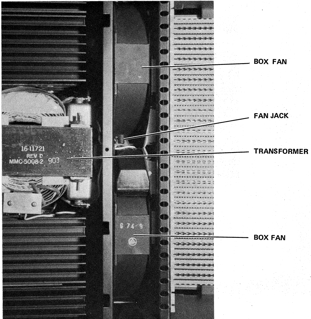
Figure 4-61 Fan Removal
