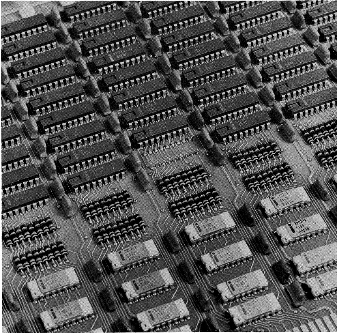
Figure B-5 Defective IC Removed
