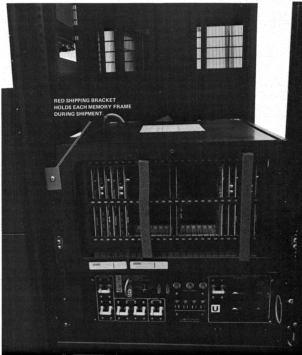
Figure 3-2 Front View of Memory Cabinet as Shipped
