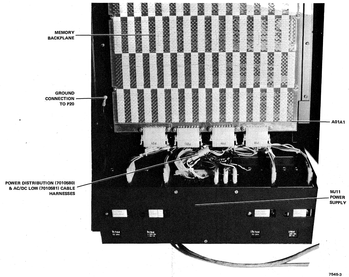
Figure 4-19 Memory Cabinet Power Supply (Bottom View)
