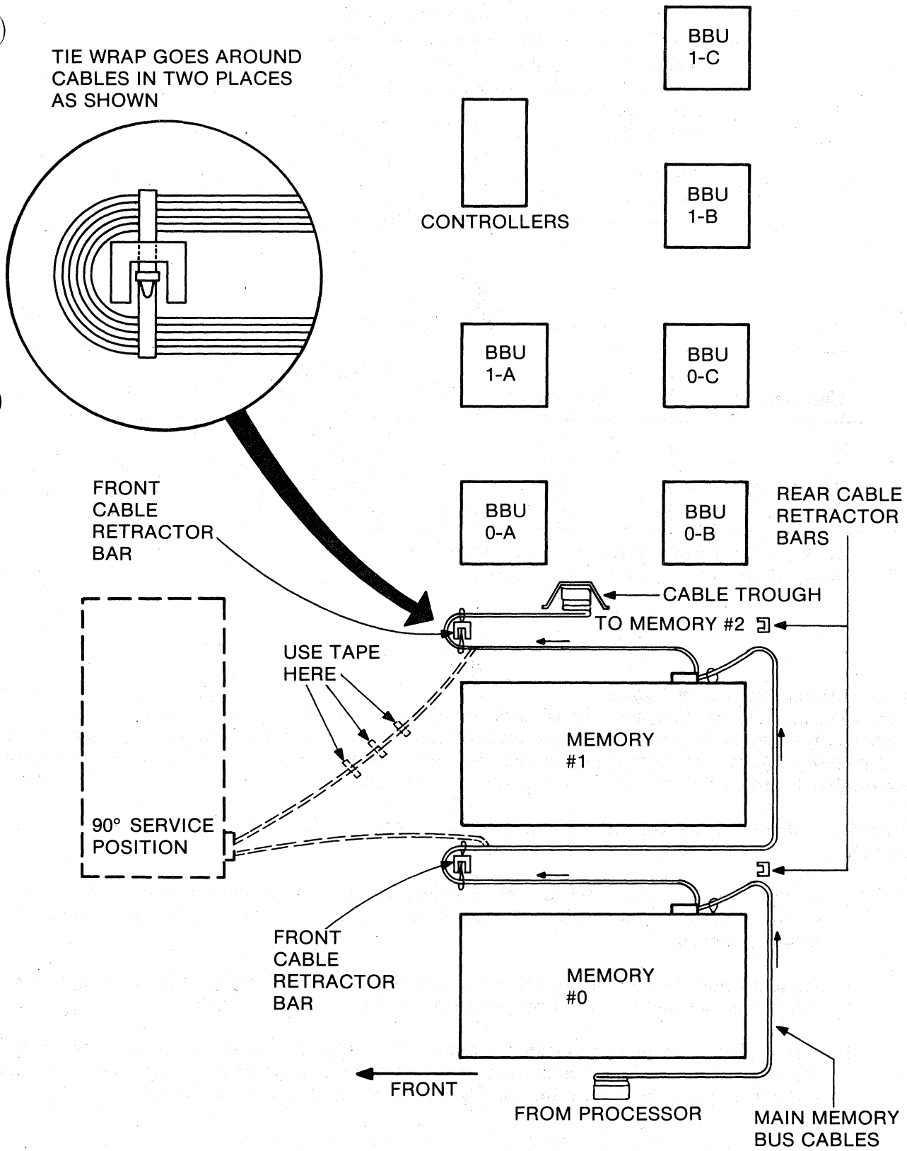
Figure 3-28 Main Memory Bus Cable Routing, First Memory Cabinet
