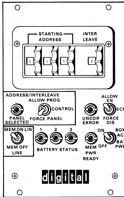
Figure 5-10 Box Controller
