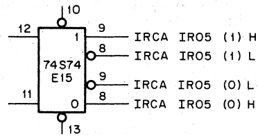
Figure 1-5 PDP-11/70 Drawing Convention Examples
