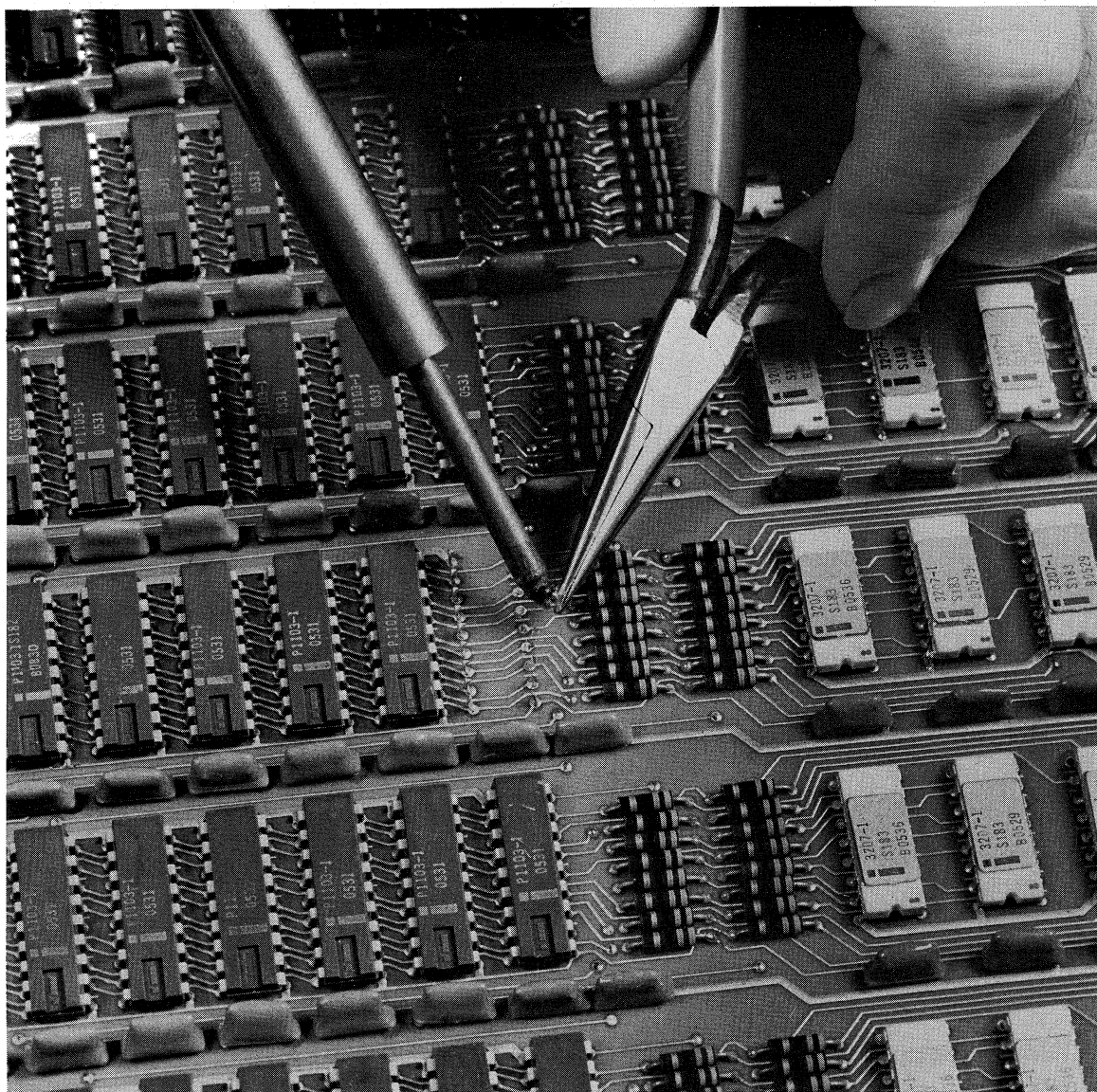
Figure B-7 IC Lead Removed
