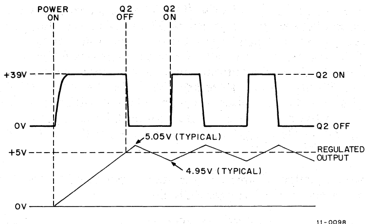
Figure 4-39 H744 Regulator Waveforms
