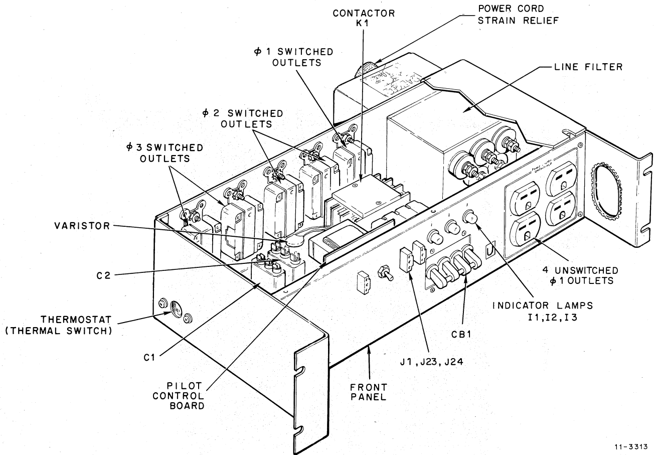
Figure 4-47 Model 861-E Power Control Component Identification
