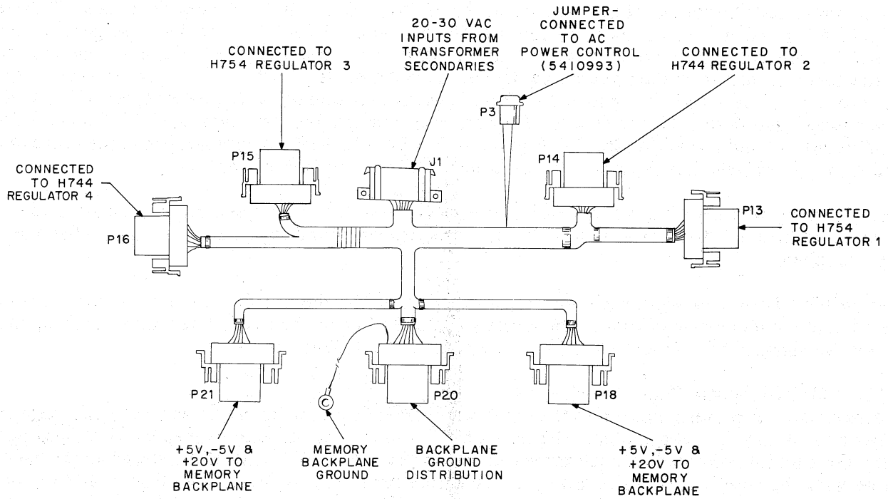
Power Harness Assembly 5010580
