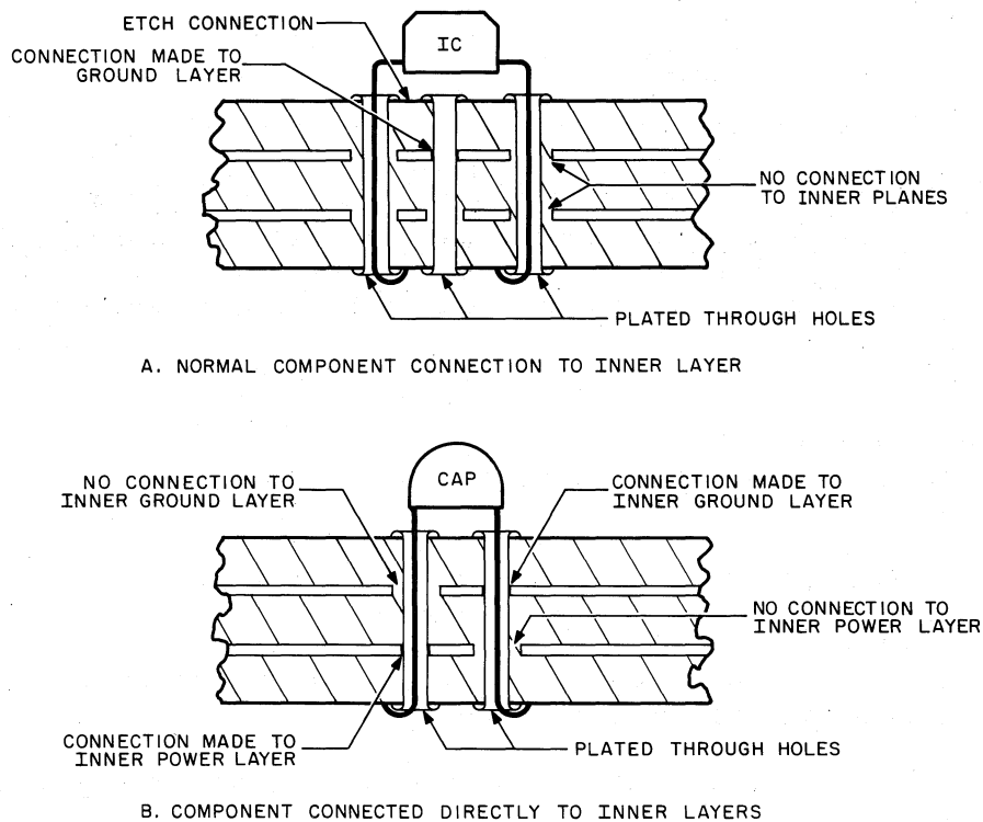
Figure B-2 Component Connections to Inner Layers
