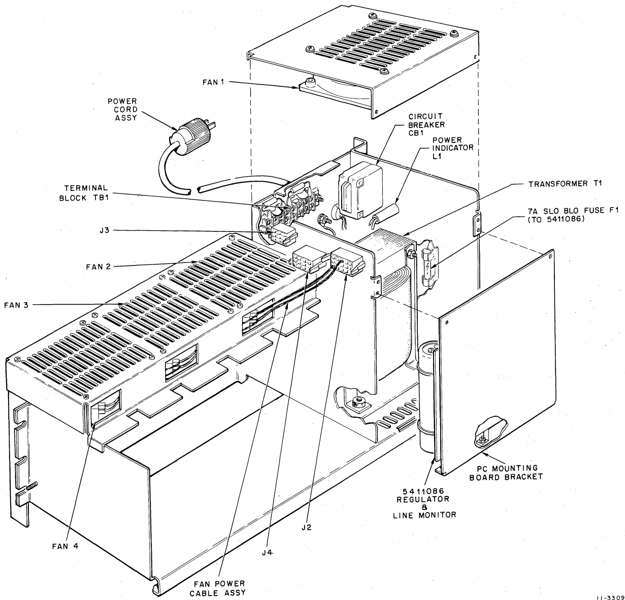
Figure 4-65 H7420 Power Supply Component Identification
