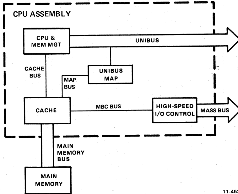
Figure 1-2 Block Diagram of PDP-11/70
