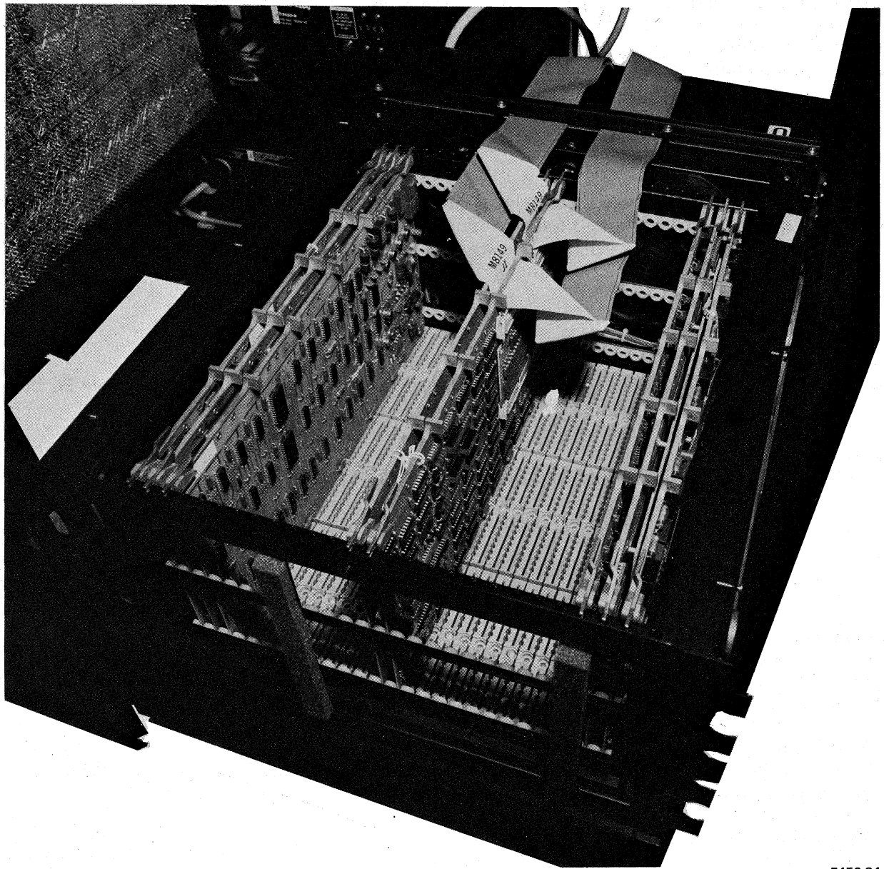
Figure 5-4 MJ11 Frame Cabling
