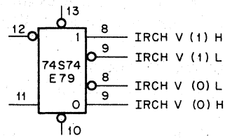
Figure 1-5 PDP-11/70 Drawing Convention Examples
