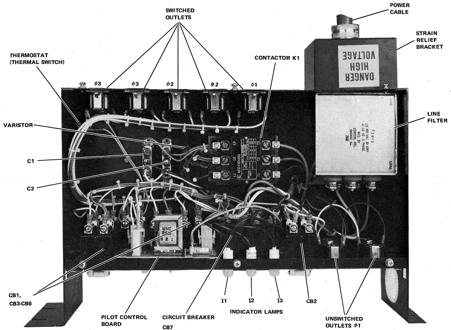
Figure 4-46 861-D Power Control Component Identification
