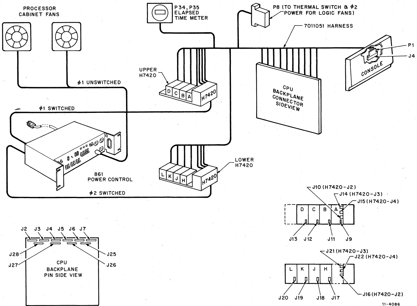
Figure 4-3 Processor Cabinet Power Connections
