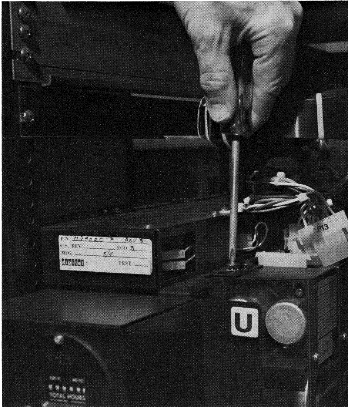
Figure 4-66 H7420 Regulator Removal (Sheet 1 of 2)
