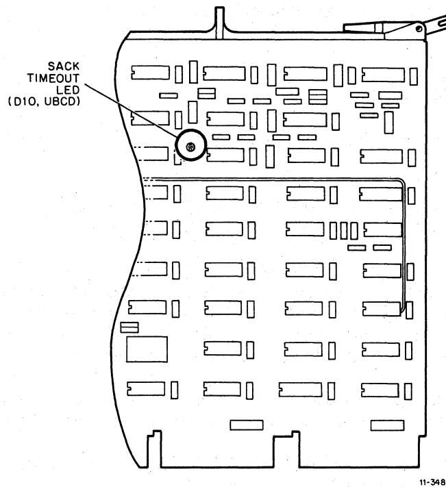
Figure 5-5 M8136 SACK Timeout LED
