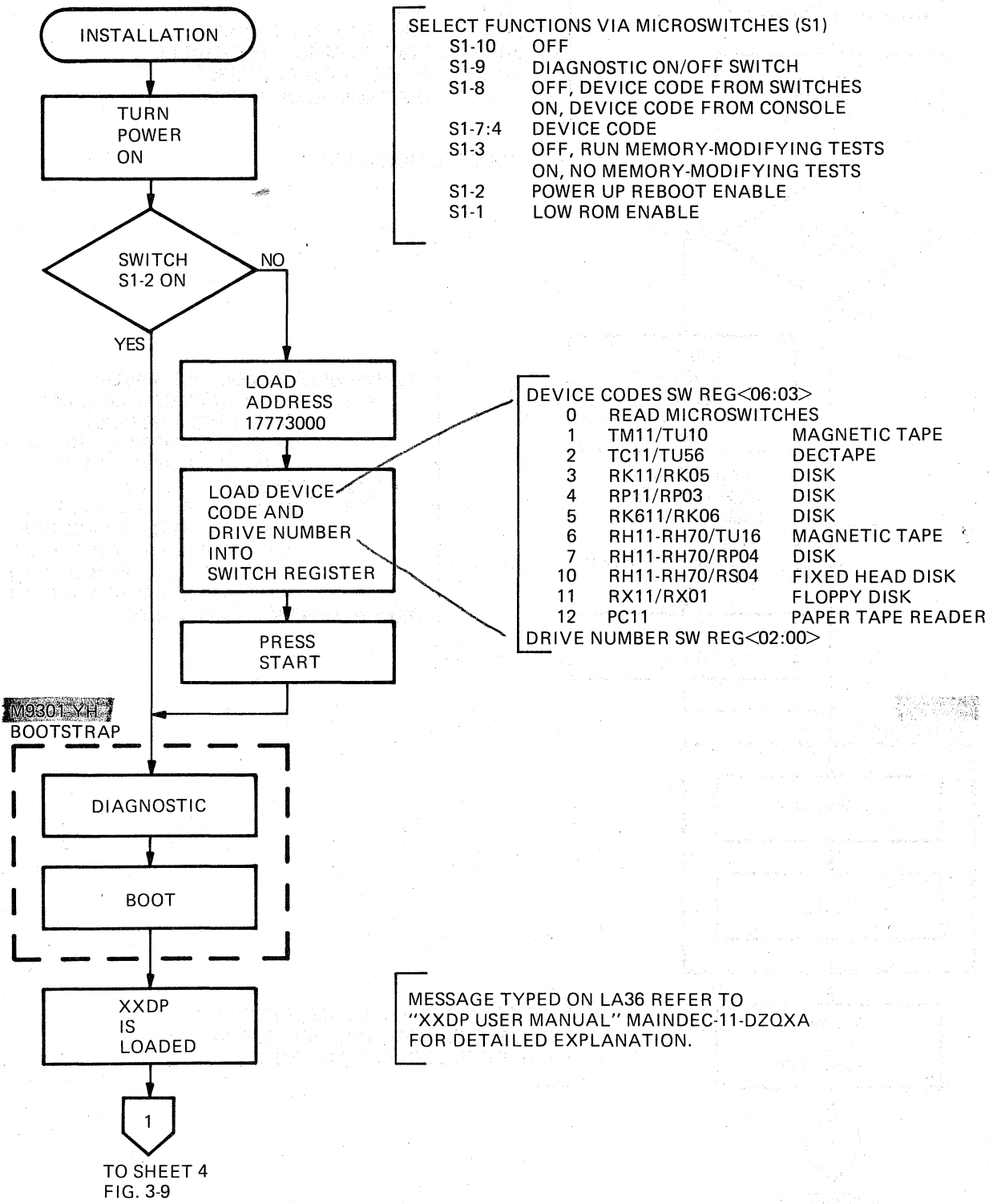
Figure 3-9 System Checkout (Sheet 2 of 4)
