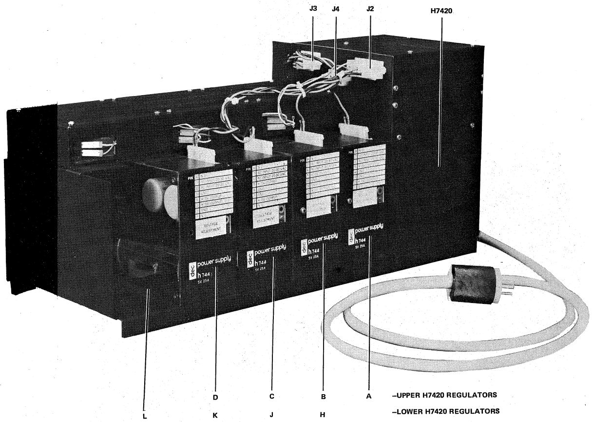
Figure 4-25 H7420 Power Supply with Regulators
