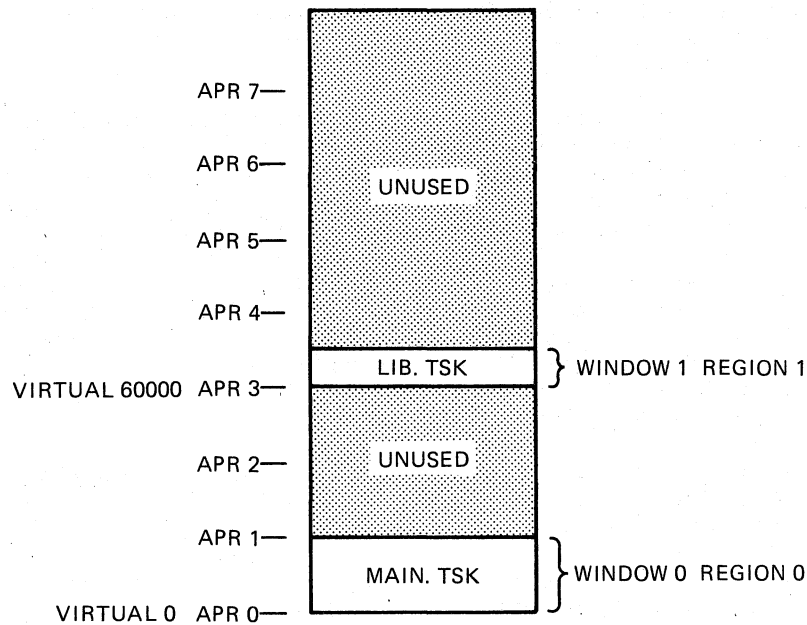
Figure 5-10 Allocation of Virtual Address Space for MAIN.TSK
