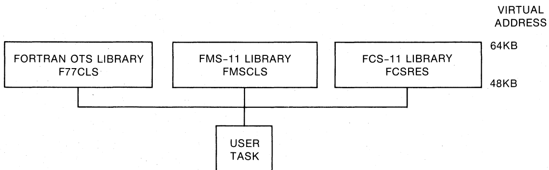
Figure 5-11 Example Library and Task Structure
