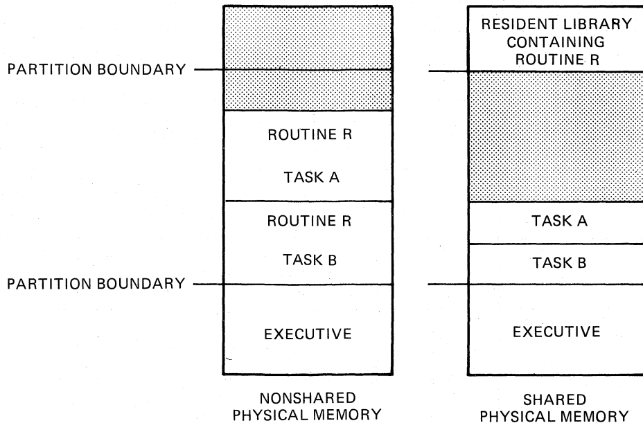
Figure 5-2 Typical Resident Library
