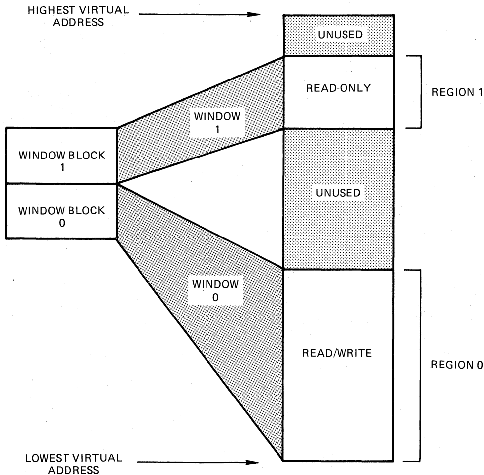
Figure 9-2 Windows for a Multiuser Task
