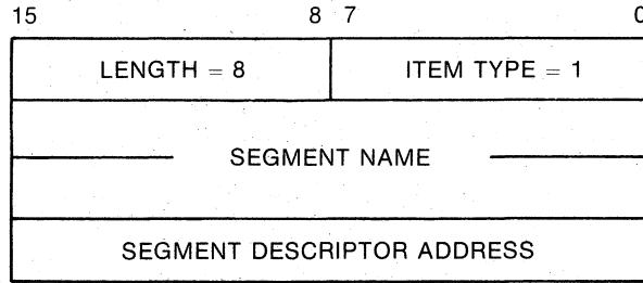
Figure A-32 Format of TKB Generated Start-of-Segment Item (1)
