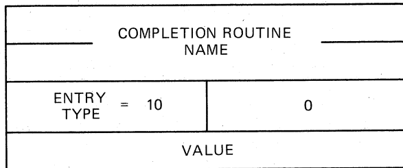
Figure A-11 Completion Routine Entry Format
