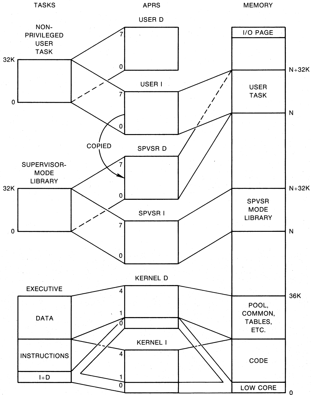
Figure 2-16 Mapping for a Conventional User Task Using a Supervisor-Mode Library in an RSX-11M-PLUS System
