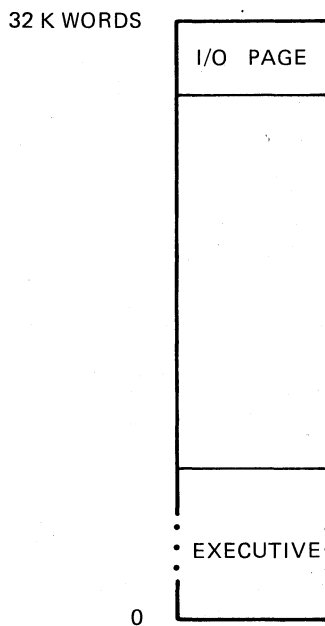
Figure 2-9 Memory Layout for Unmapped System
