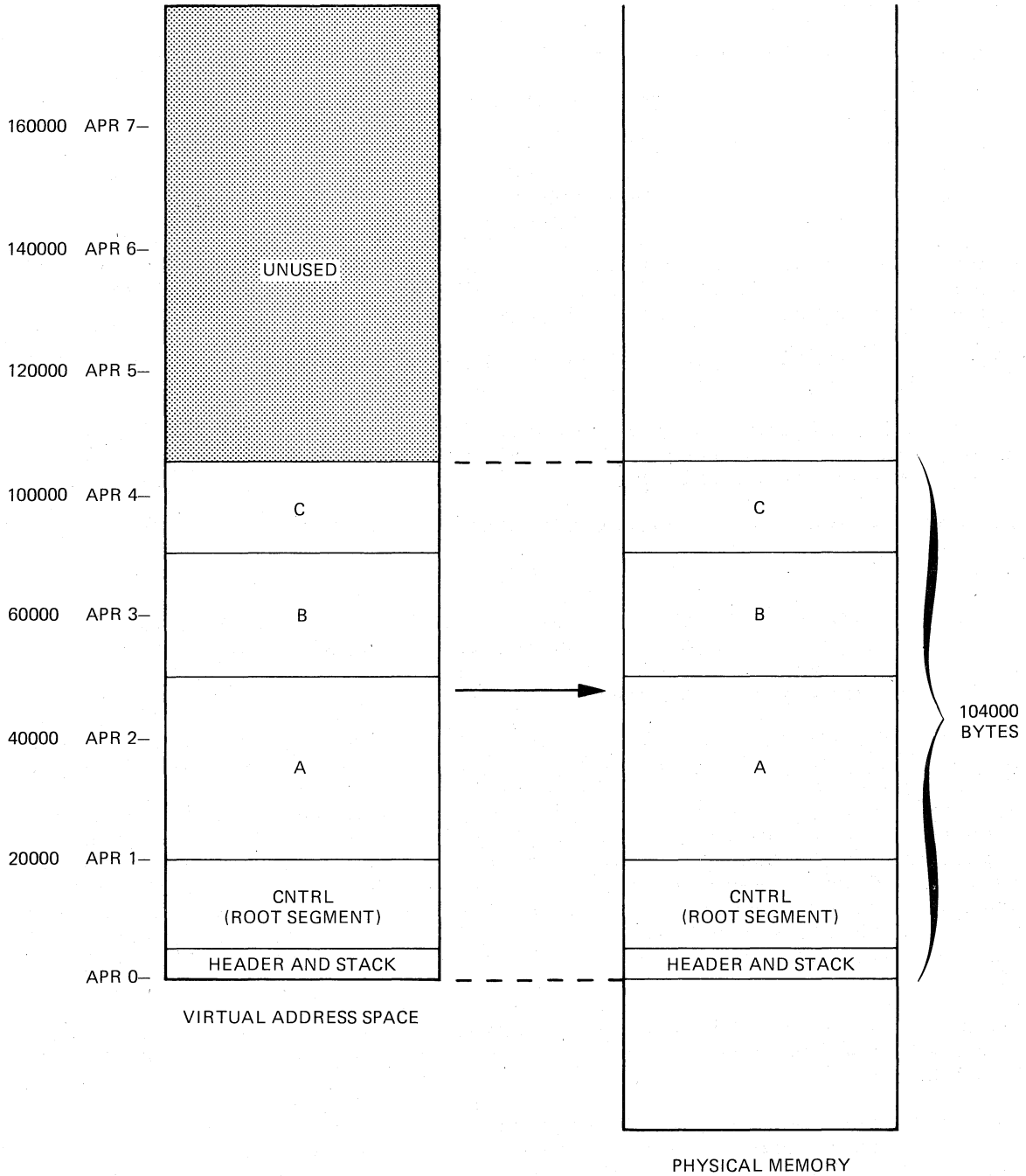
Figure 3-1 TK1 Built As a Single-Segment Task
