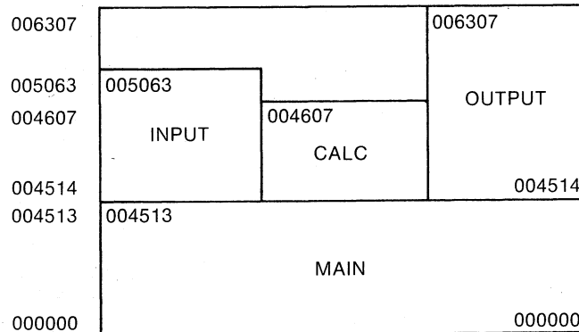
Figure 7-7 Memory Allocation Diagram for MAIN.TSK
