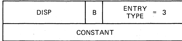
Figure A-17 Internal Displaced Relocation Entry Format
