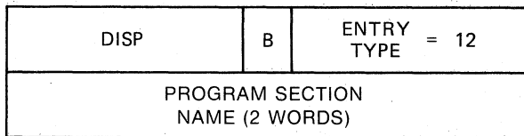
Figure A-24 Program Section Relocation Entry Format
