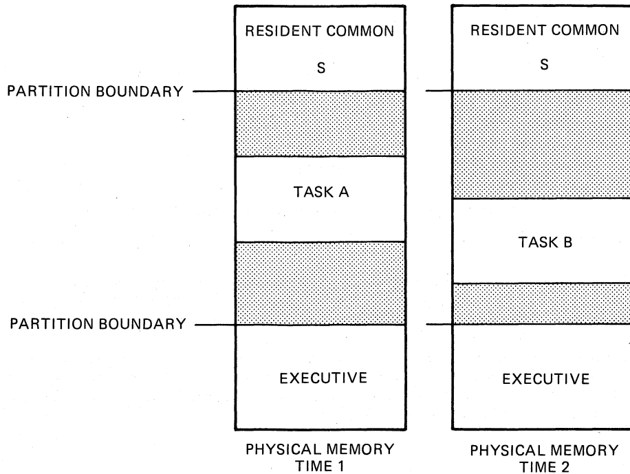
Figure 5-1 Typical Resident Common
