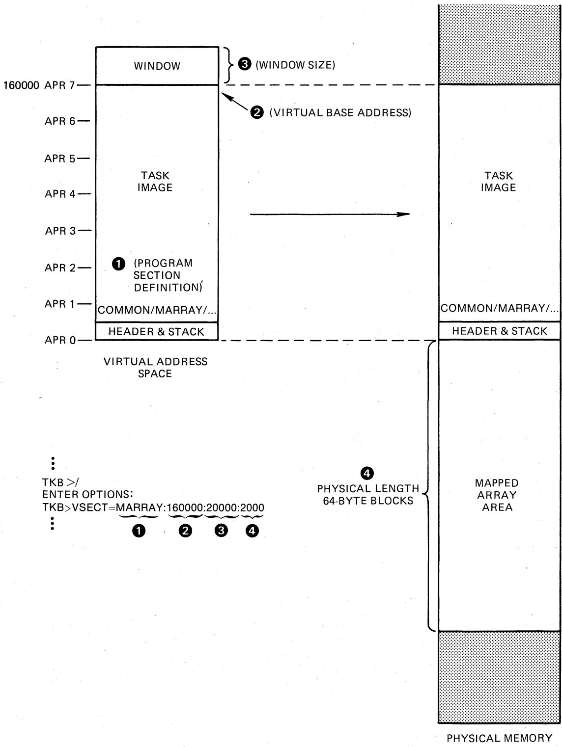
Figure 5-15 VSECT Option Usage
