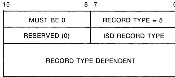
Figure A-30 General Format of All ISD Records
