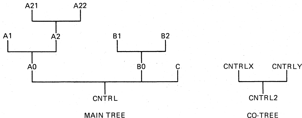
Figure 3-16 Overlay Co-Tree for Modified TK1
