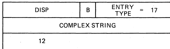
Figure A-28 Complex Relocation Entry Format
