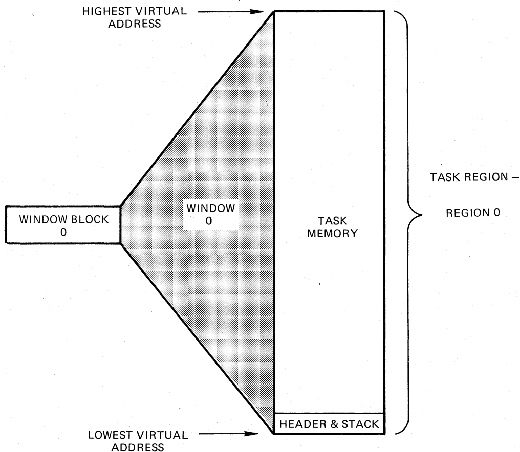
Figure 2-13 Window Block 0
