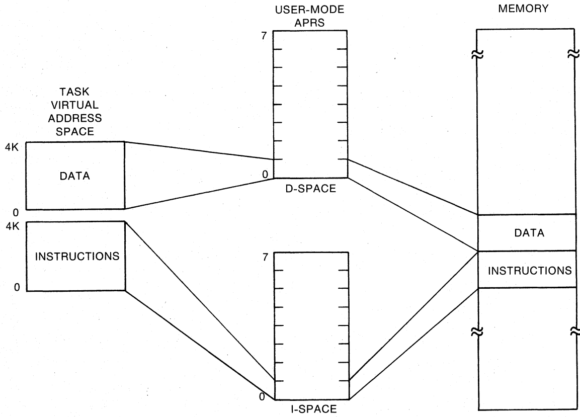
Figure 2-17 Simplified APB Mapping for an I- and D-space Task
