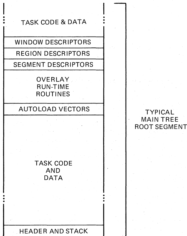
Figure 3-11 Typical Overlay Root Segment Structure
