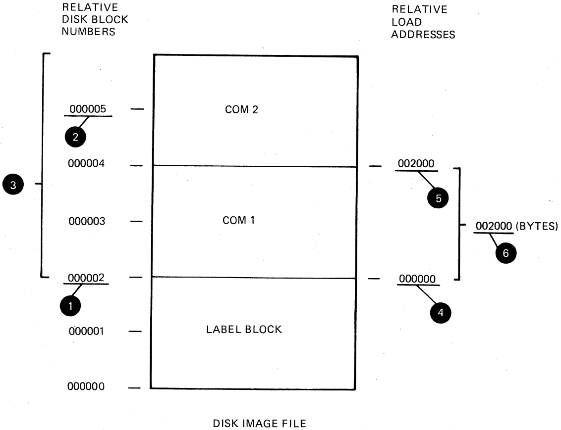
Figure 5-8 Allocation Diagram for MACCOM.TSK
