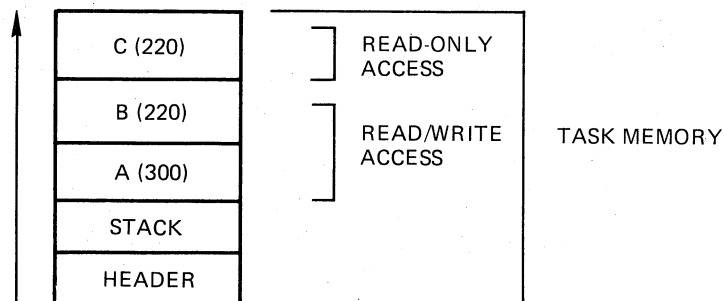
Figure 2-3 Allocation of Task Memory
