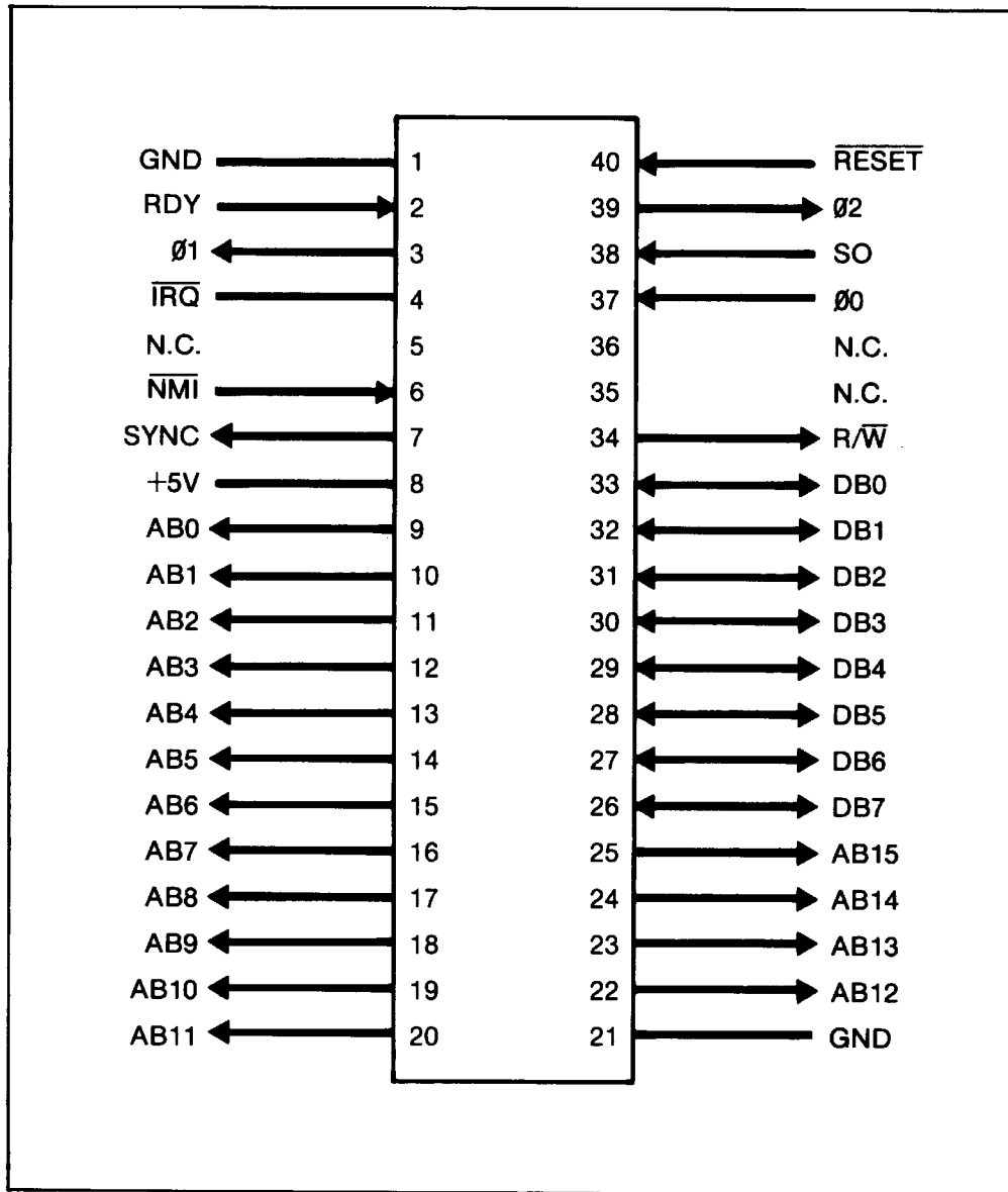
Figure 3-1. 6502 Pin Assignments
