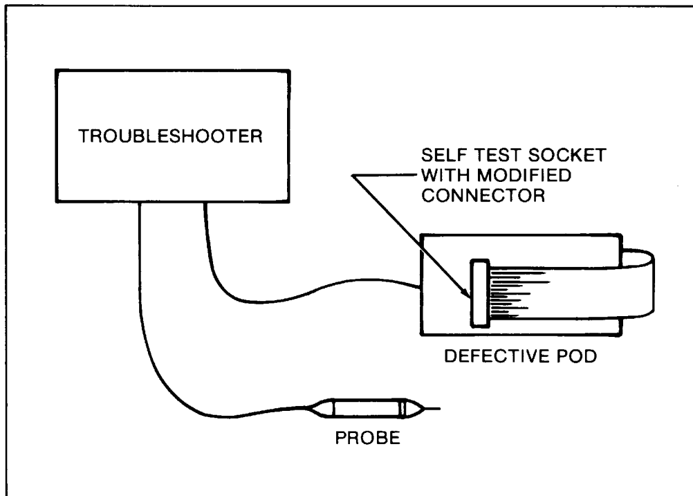
Figure 5-2. Troubleshooting a Defective Pod
