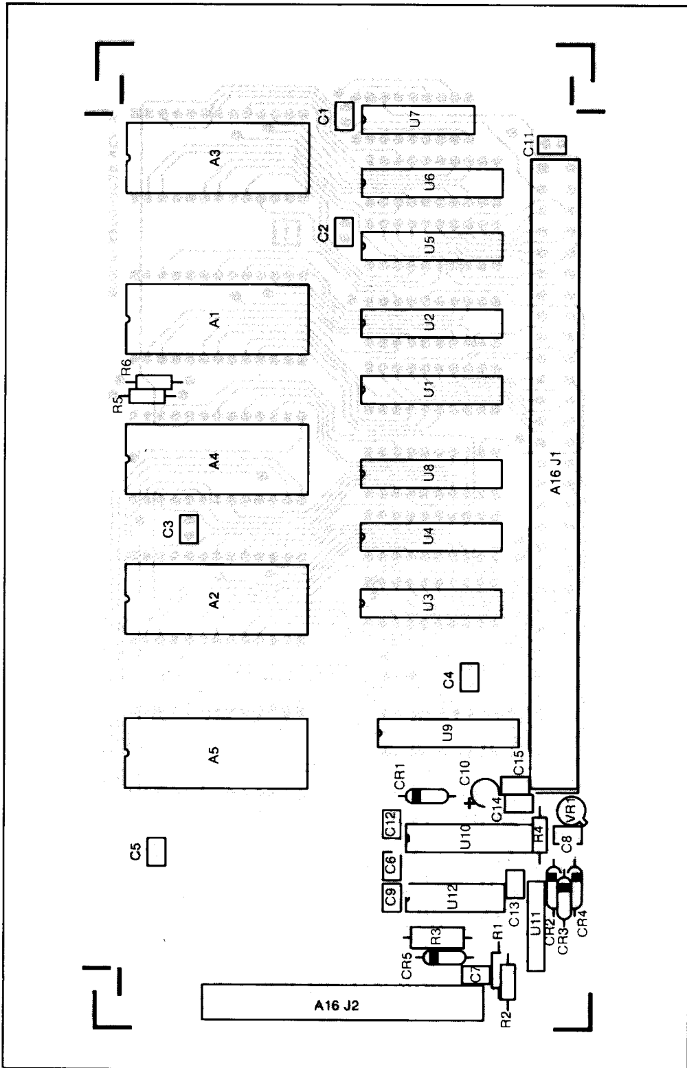
Figure 5-1. Interface PCB, Non-Component Side
