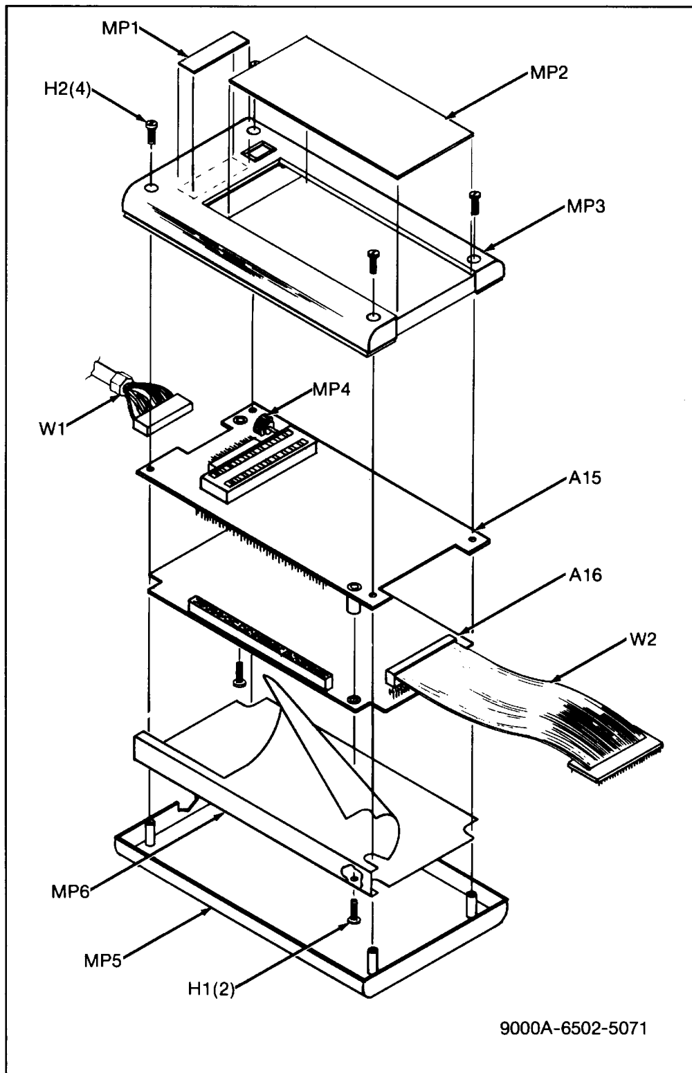
Figure 6-1. 9000A-6502 Interface Pod Final Assembly
