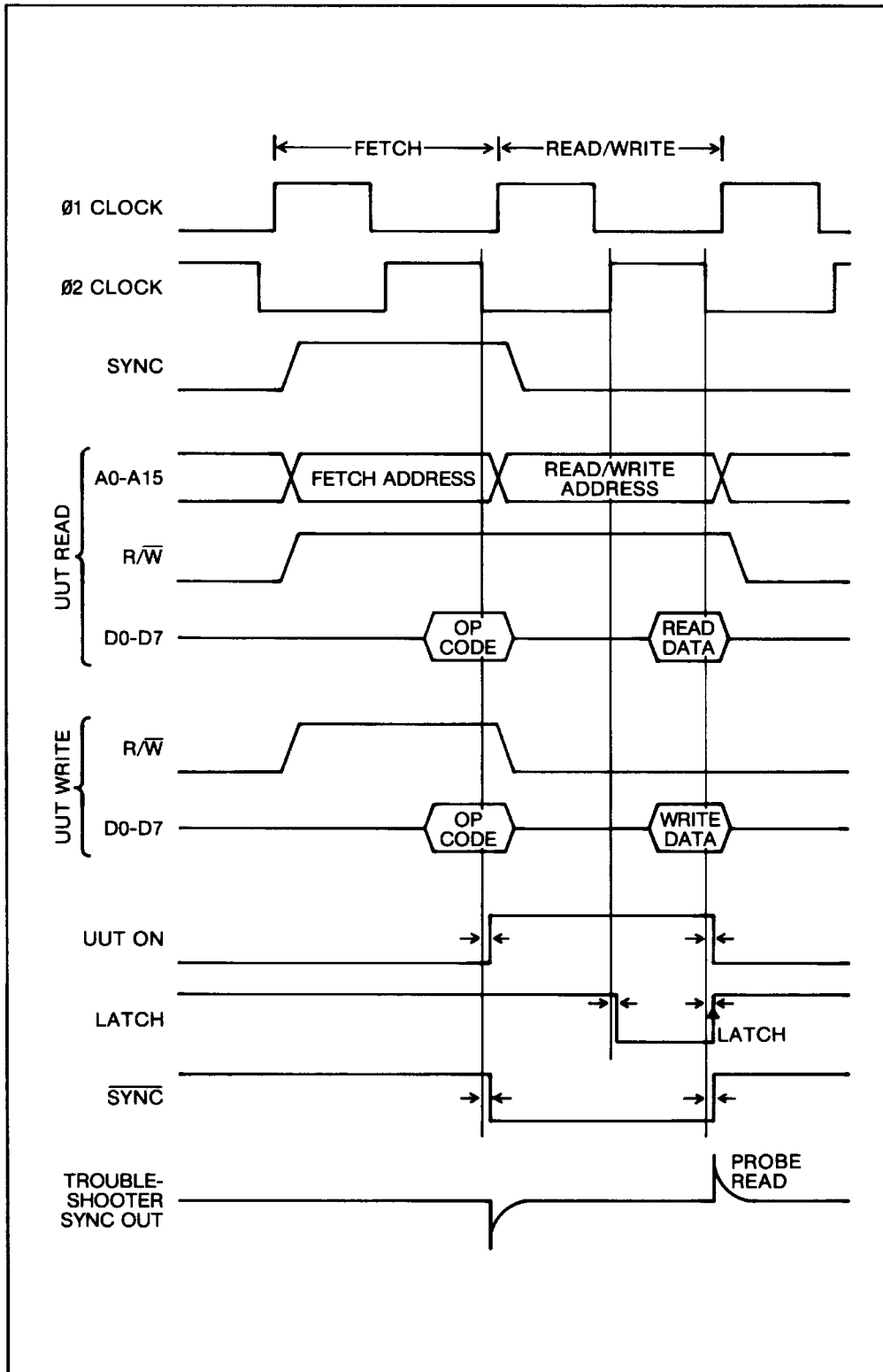
Figure 4-4. UUT ON Signal and Latch Times
