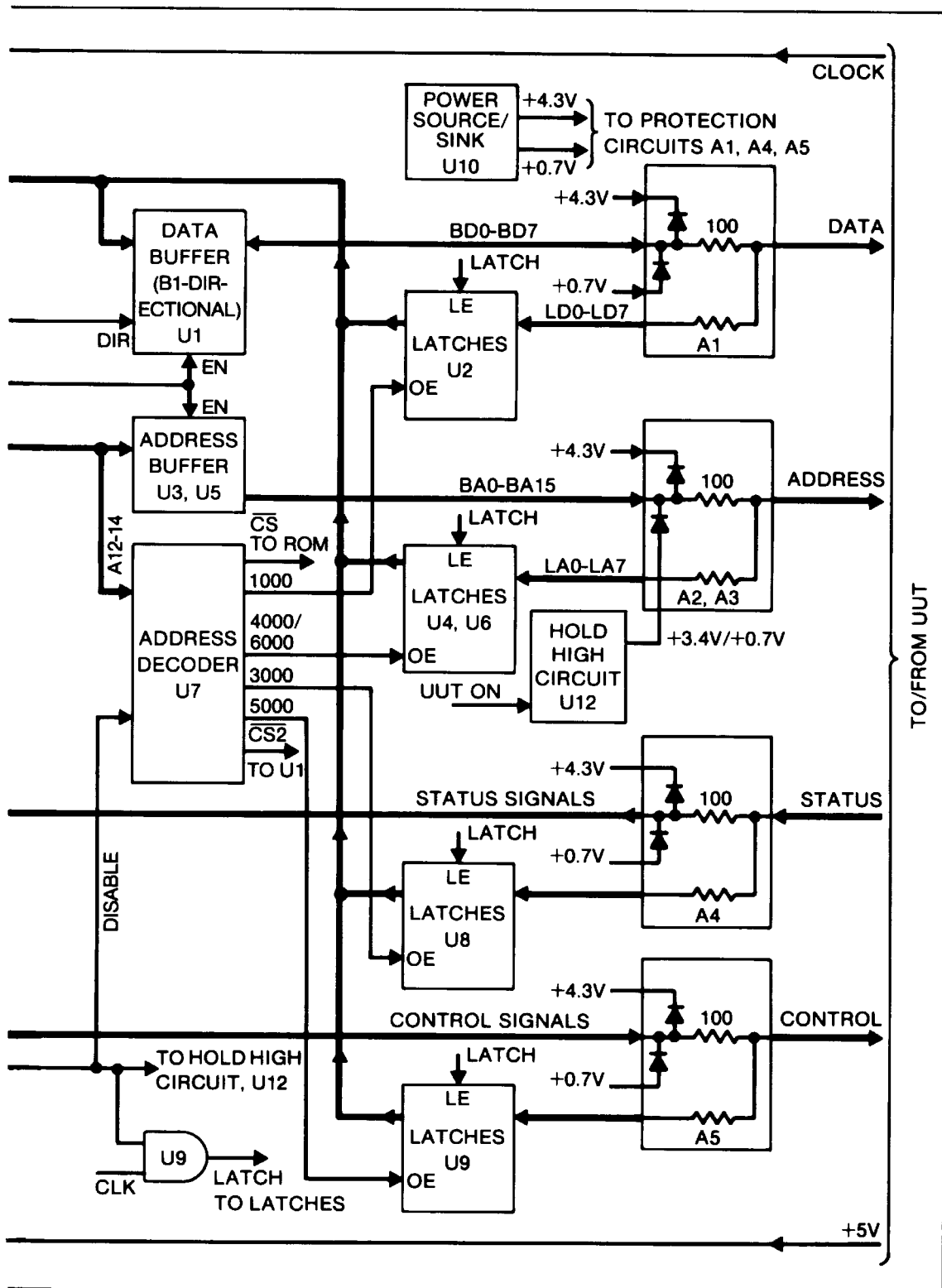
Figure 4-2. Detailed Block Diagram
