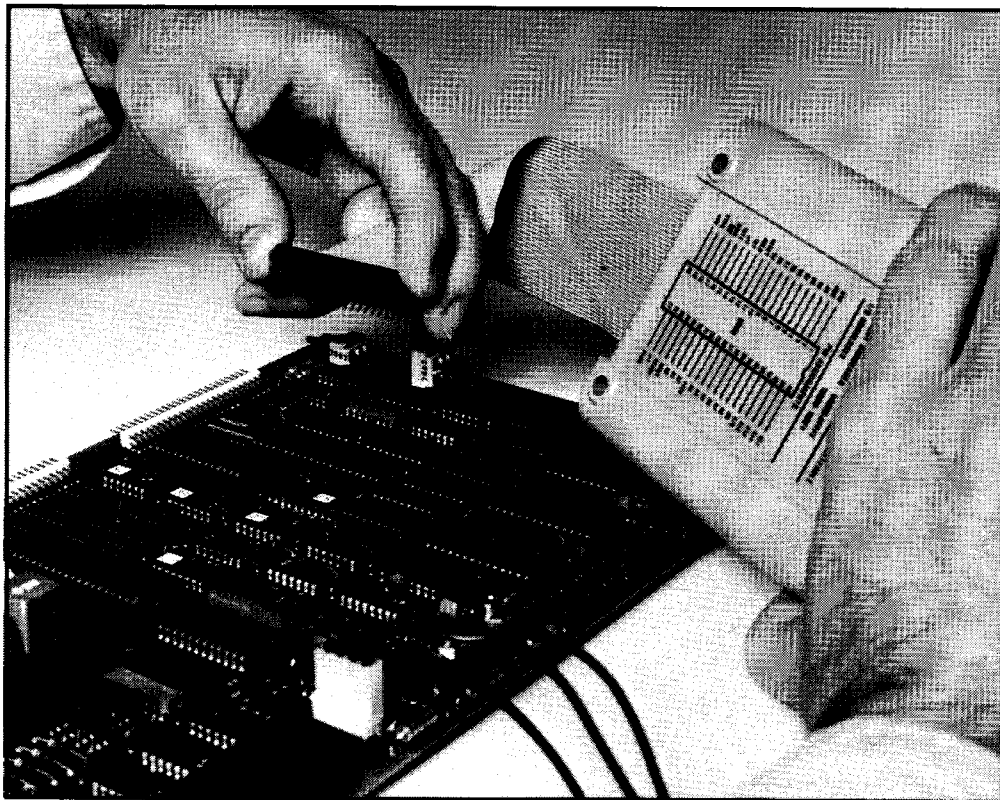
Figure 2-2. Connection of Interface Pod to UUT
