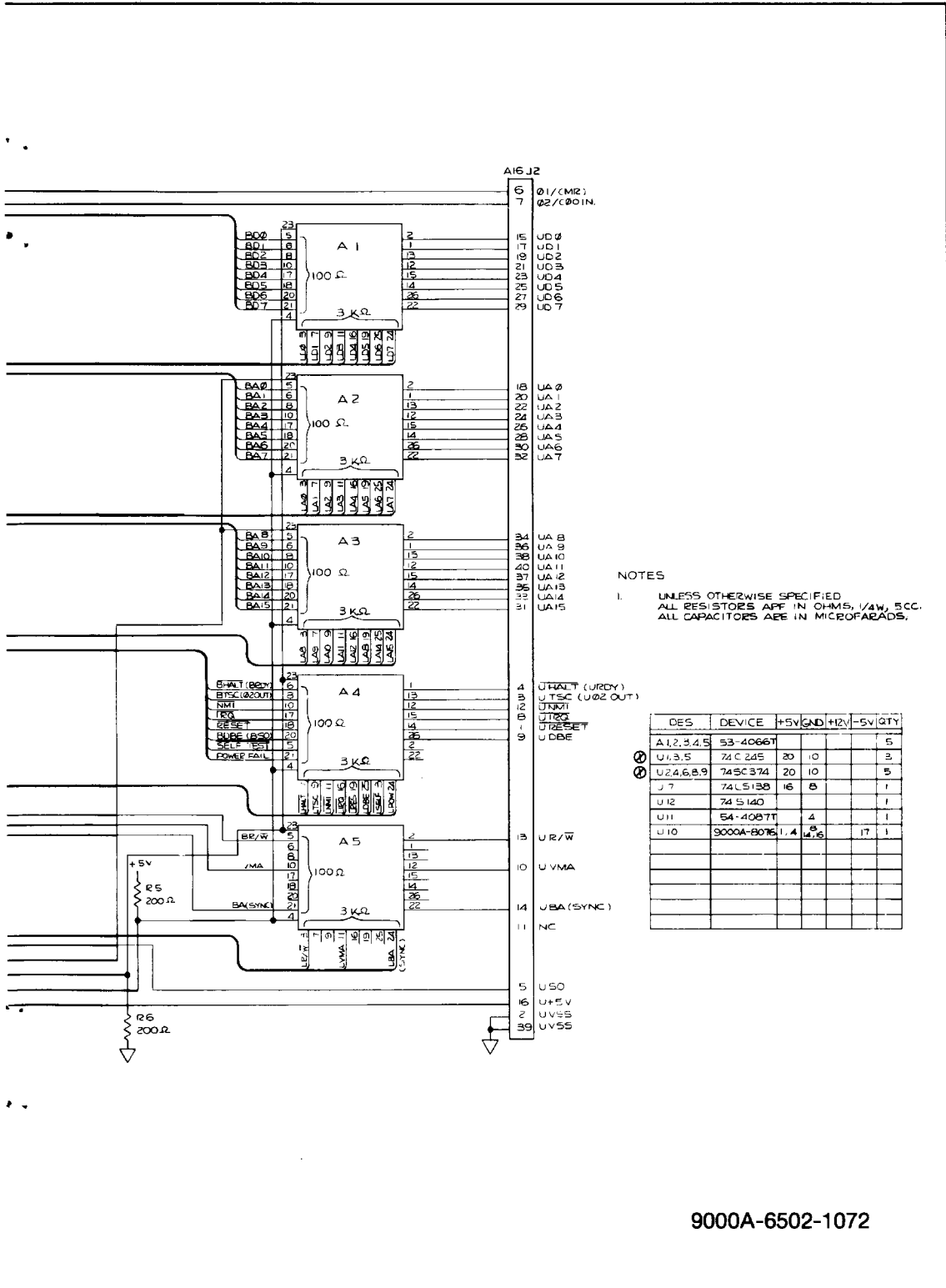
Figure 7-2. A16 Interface PCB Assembly
