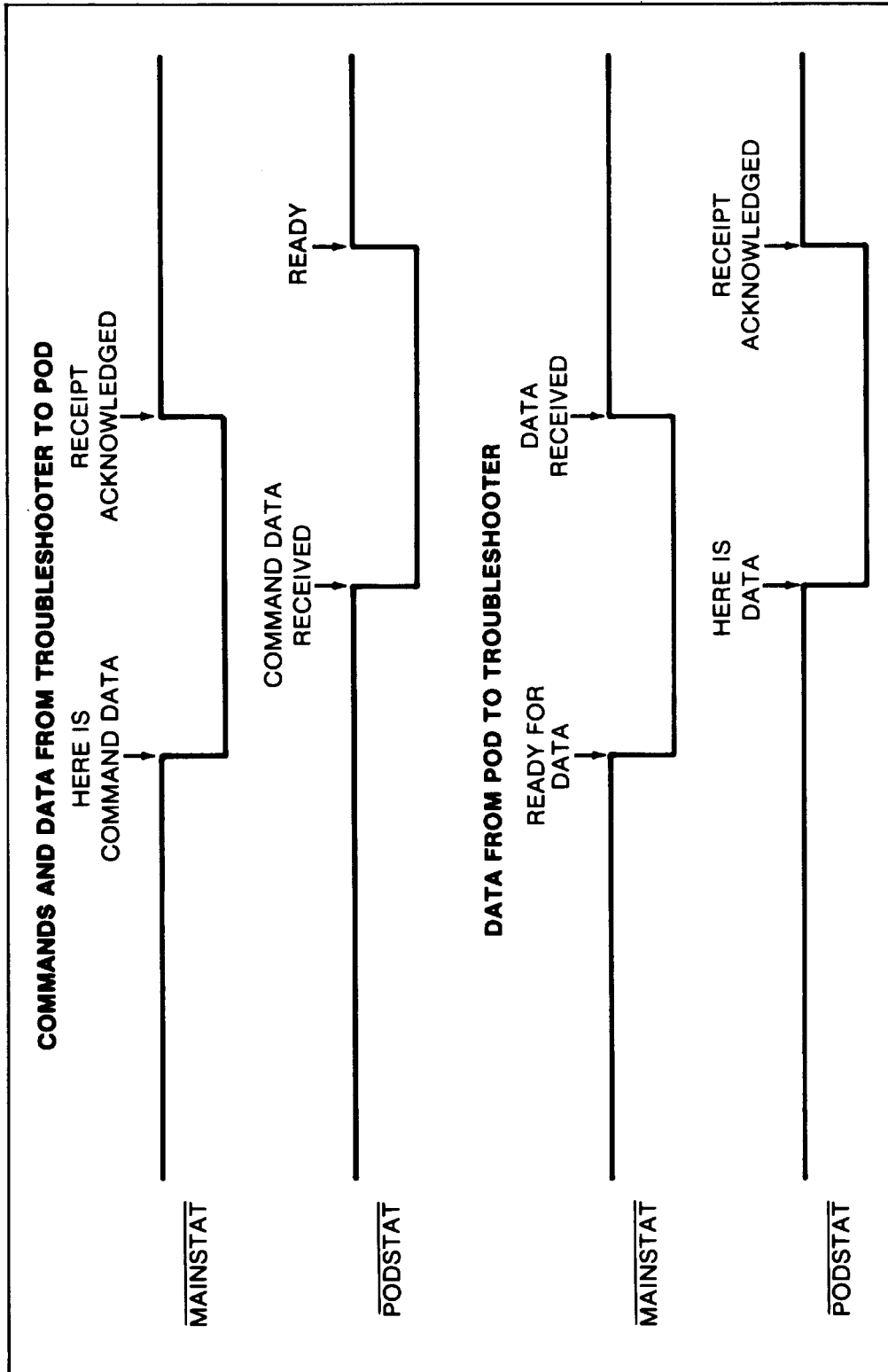
Figure 4-3. Handshaking Signals
