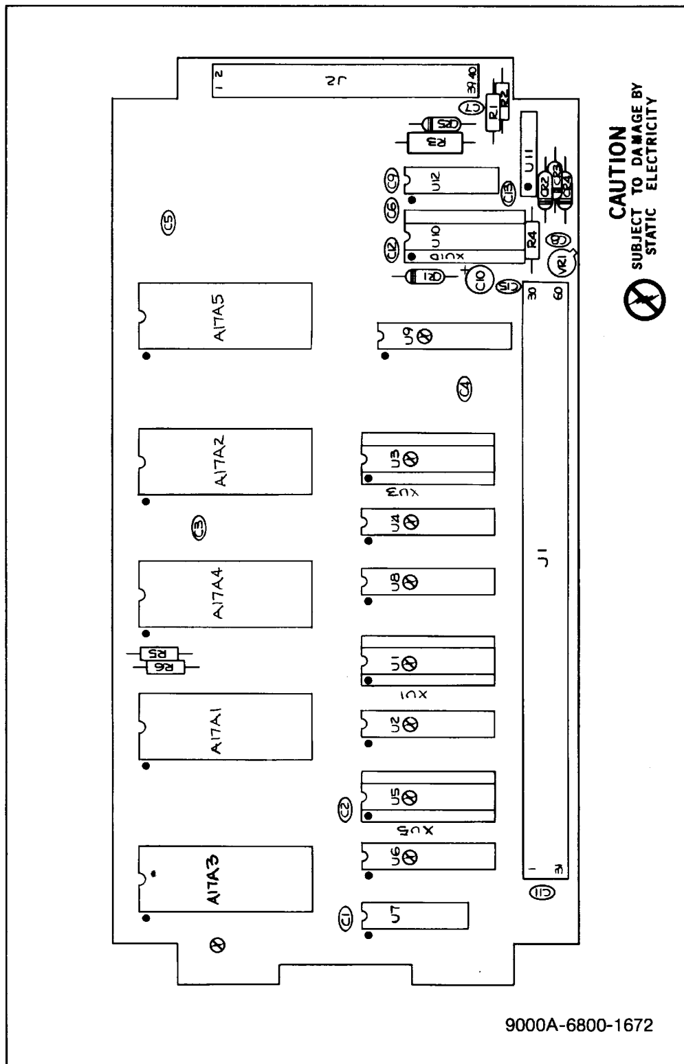
Figure 6-3. A16 Interface PCB Assembly
