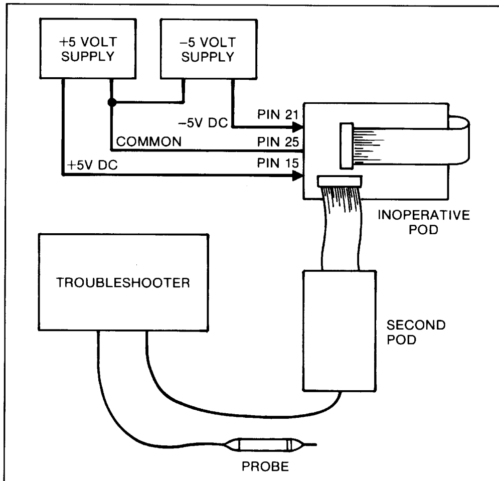
Figure 5-3. Troubleshooting an Inoperative Pod
