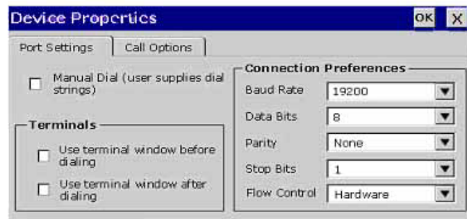
Figure 5.7 Port Settings
