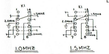
FIGURE 3-2. MPU II Module, Schematic Diagram
