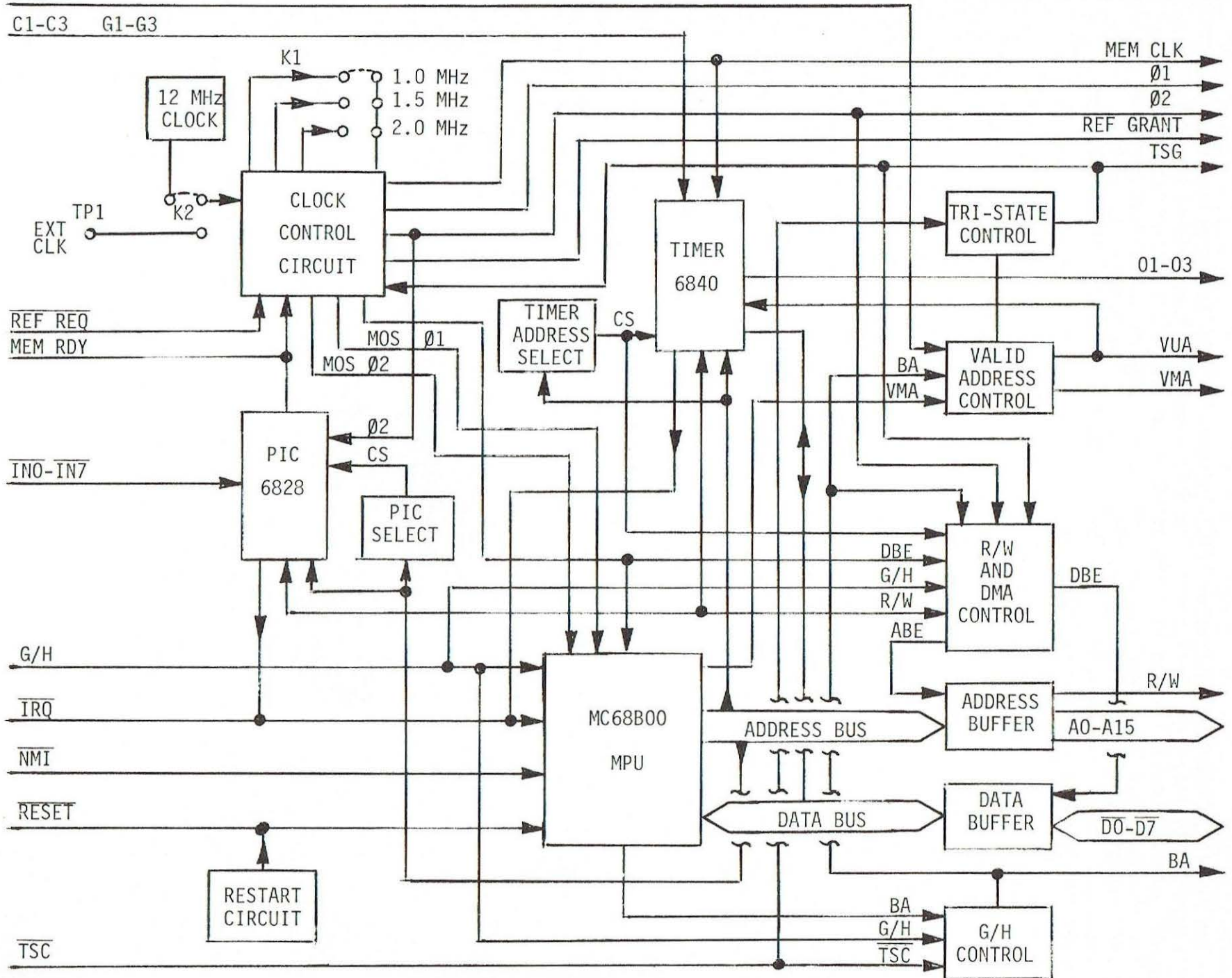
FIGURE 3-1. MPU II Module, Block Diagram
