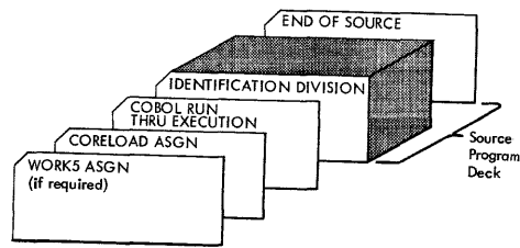
Figure 6. COBOL RUN THRU EXECUTION
