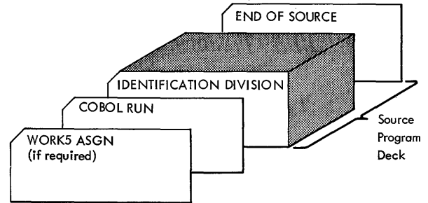
Figure 3. COBOL RUN
