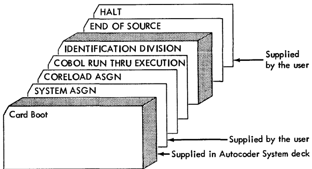
Figure 17. Sample Program
