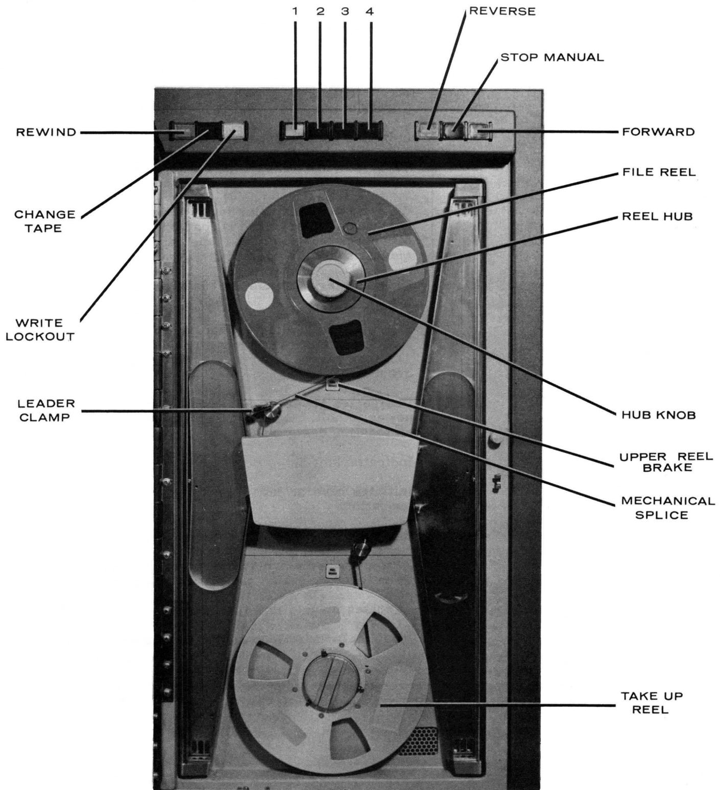
Figure 4-9. 1607 Tape Unit
