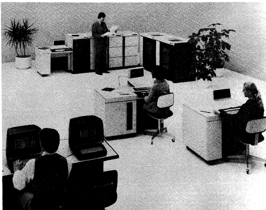
This large configuration of the Burroughs B 820 system includes, in the foreground, two TD 830 CRT's at left, a Direct Data Entry Station (DDES) at right, and an AE 500 Audit Entry Station with two Super Mini-Disk drives in the center. From left to right in the background are the DDES console, a double-width B 820 processor, two disk pack drive cabinets, and two line printers.
