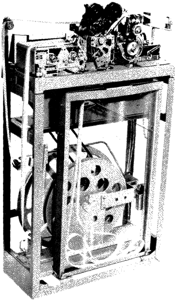
Figure 15. M28 Reperforator Transmitter (RT). An ROTR with paper tape storage facilities for buffering, and a paper tape reader for re-transmitting.
