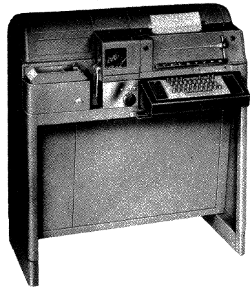
Figure 13. M28 Automatic Send-Receive Set (ASR). A half-duplex teletypewriter station which contains a page printer, keyboard, tape punch and tape reader.
