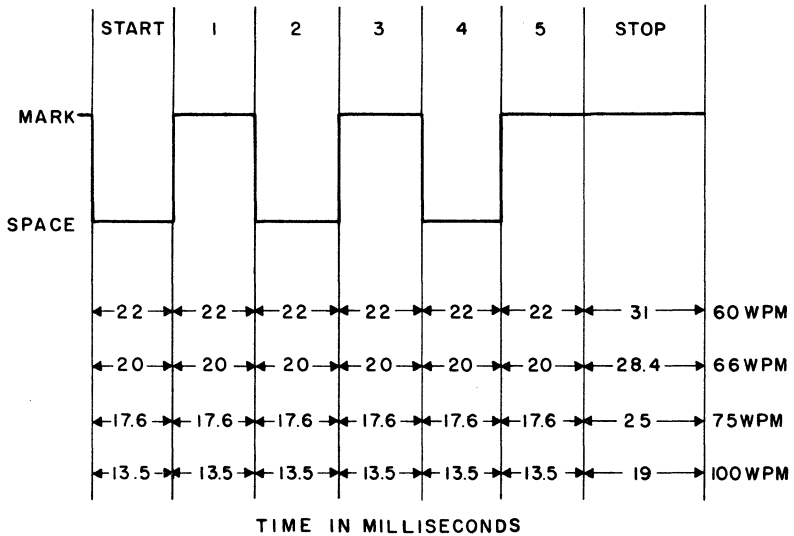
Figure 2. The 7.42 Unit Code Time Base Using the Letter Y as an Example
