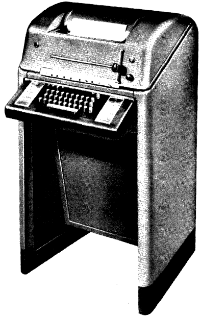
Figure 11. M28 Keyboard Send-Receive Set (KSR). A transmitter-receiver consisting of an RO with keyboard for manual sending.
