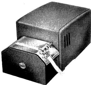
Figure 14. M28 Tape Transmitter (TD). A paper tape reader.
