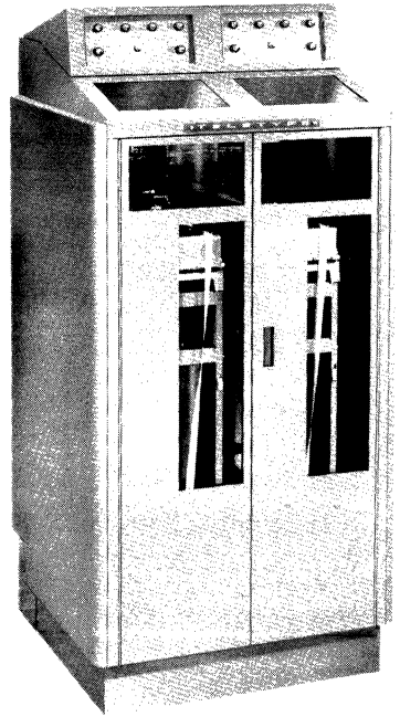
Figure 16. M28 Reperforator Transmitters (Two in One Cabinet)
