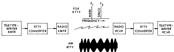
Figure 9. Simplified RTTY System
