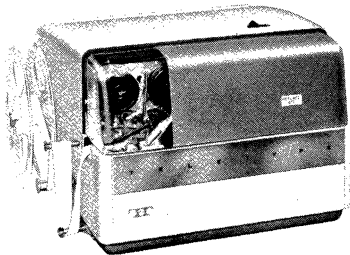
Figure 21. M35 Receive-Only Typing Reperforator. An 8-level paper tape receiver.
