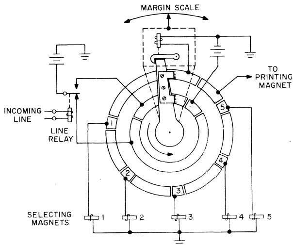
Figure 5. Receiving Distributor
