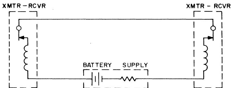
Figure 4. Half-Duplex Circuit
