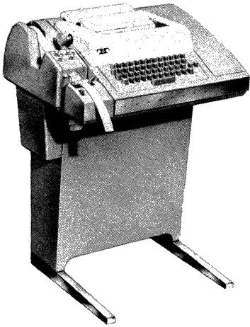
Figure 18. M33 Automatic Send-Receive Set. A standard duty 8-level ASR.
