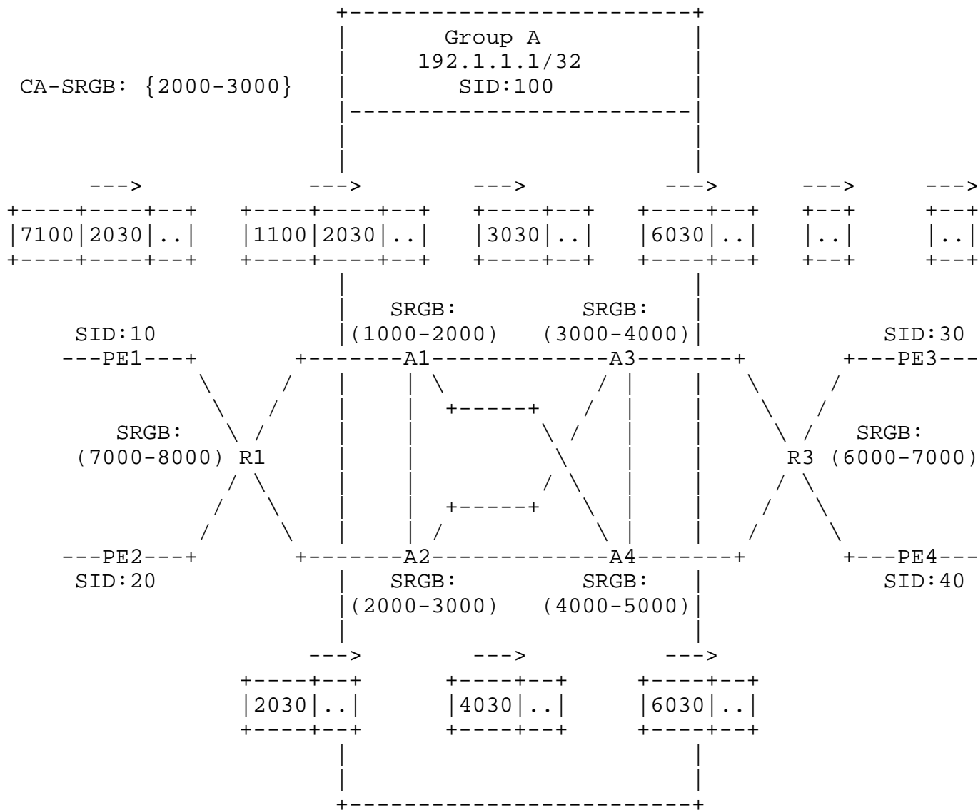
Figure 4: Packet Flow through MPLS-based SR Anycast Segments
