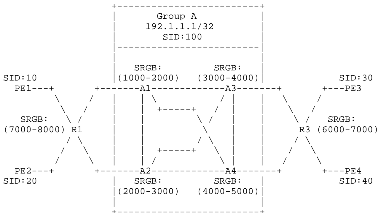
Figure 2: Transit paths via anycast group A
